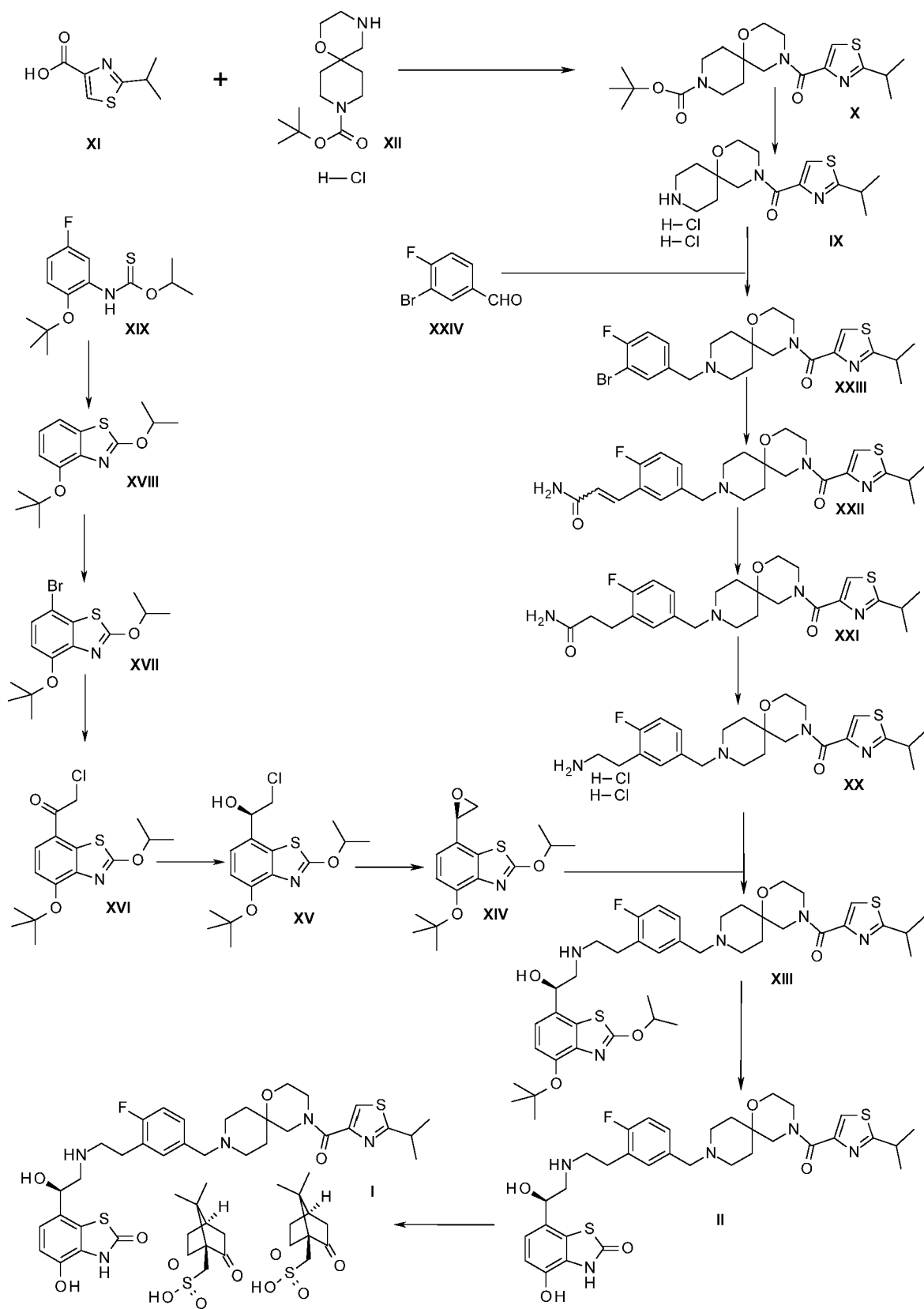
Scheme 2
