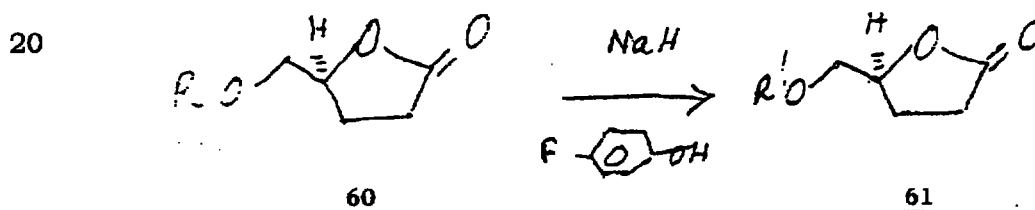
Scheme XIV
