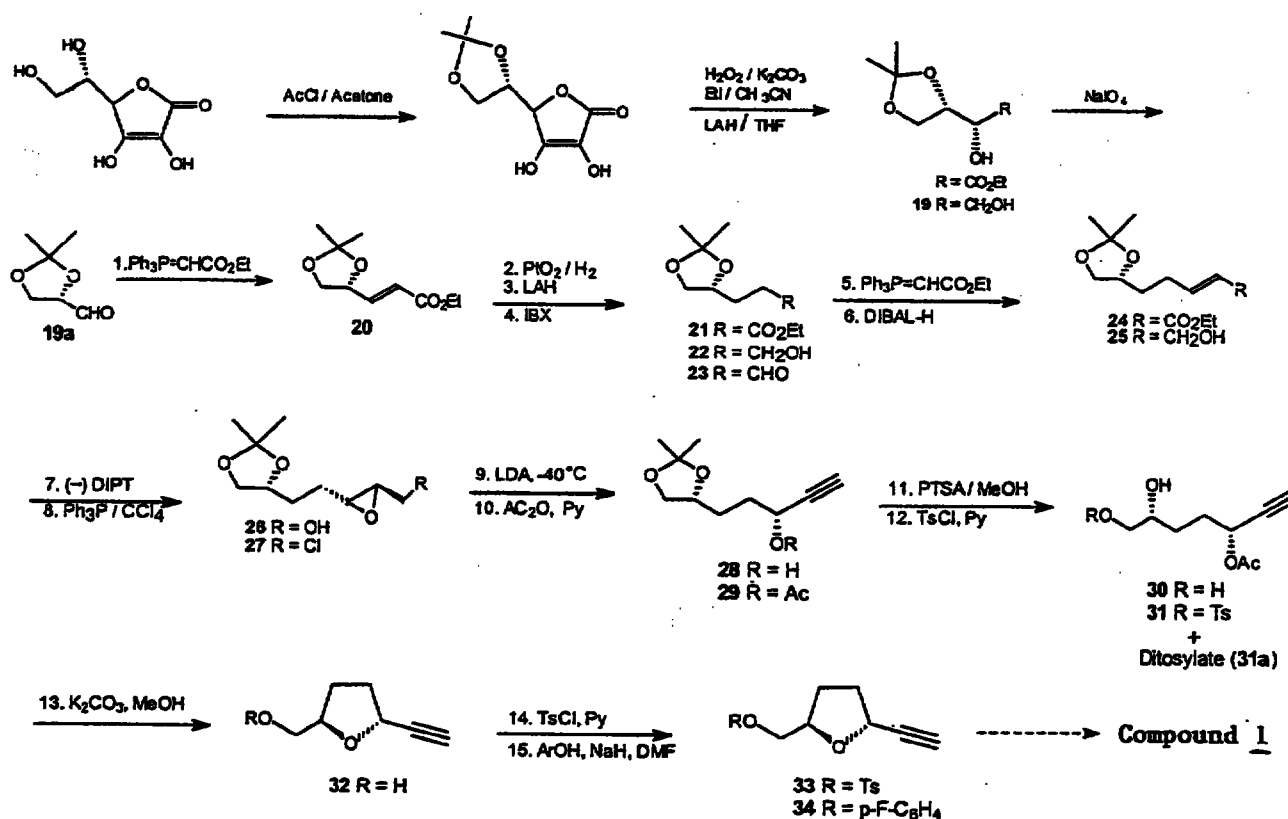
Scheme IX
