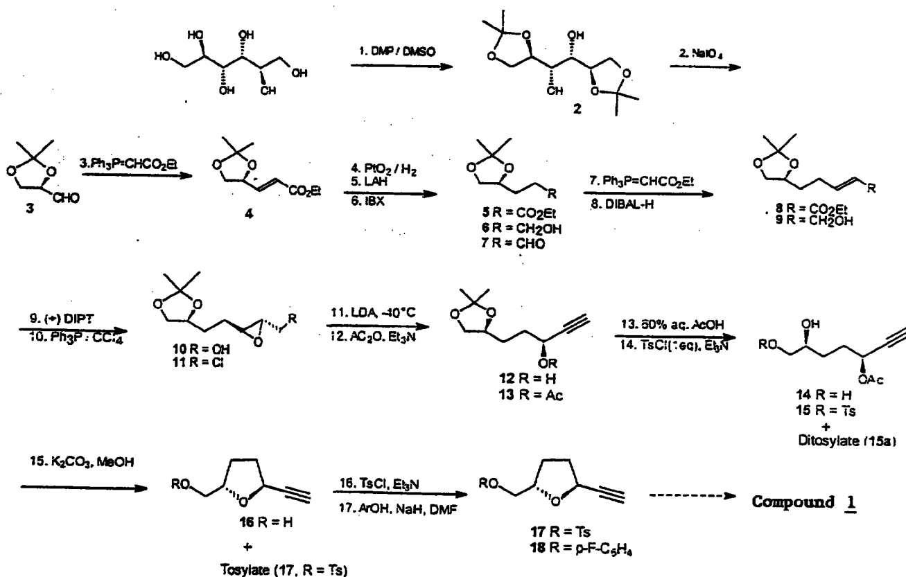
Scheme VIII
