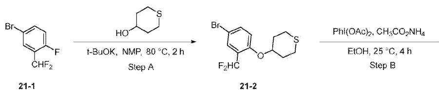
Compound 234
