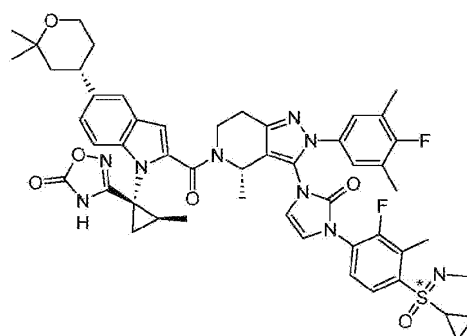
Compound 196
