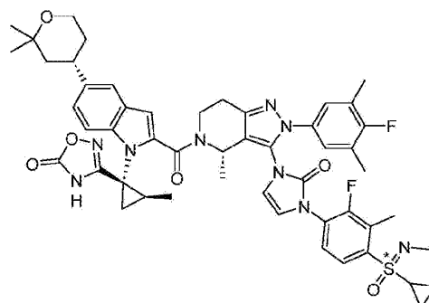
Compound 196
