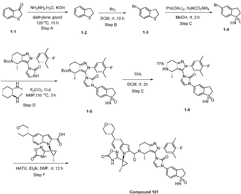
Compound 101
