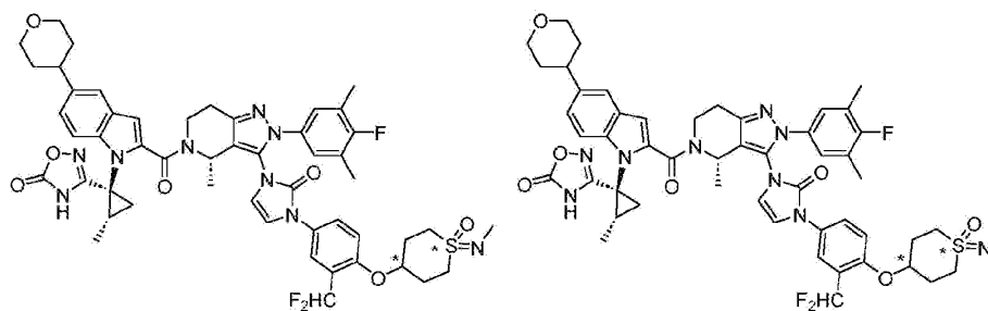
Compound 234
