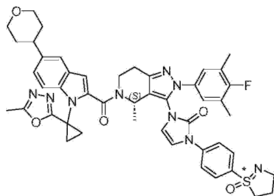
Compound 156
