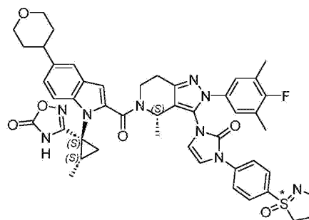
Compound 143 enantiomer 2
