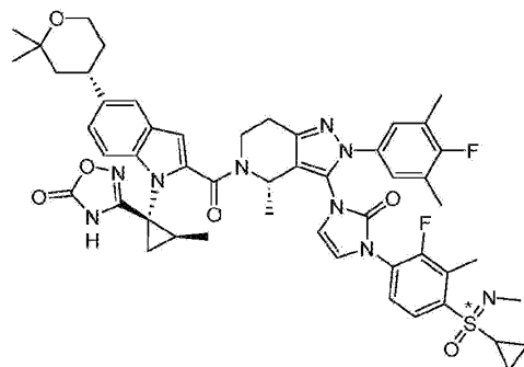
Compound 195
