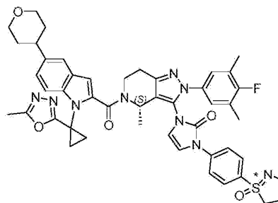
Compound 155
