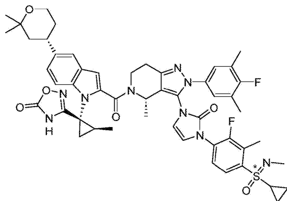
Compound 195
