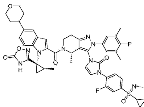
Compound 222
