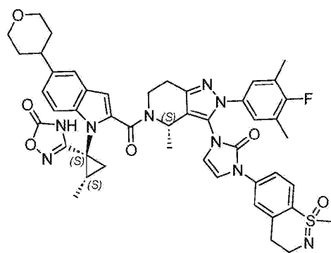
Compound 108
