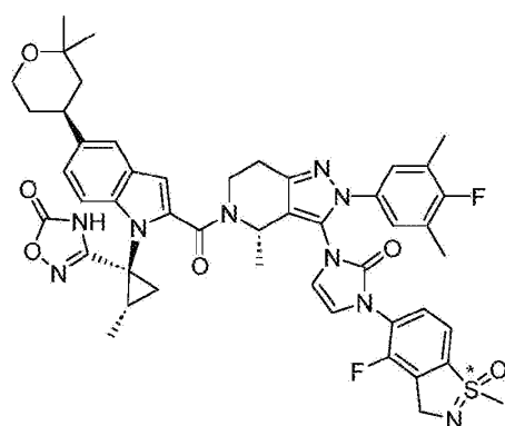
Compound 187
