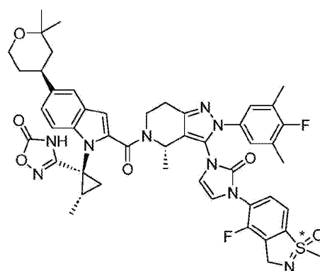
Compound 188
