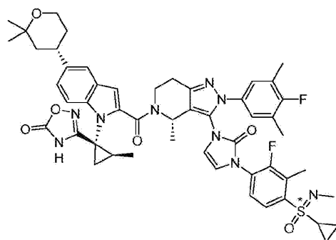
Compound 195
