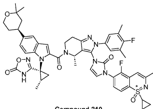
Compound 210
