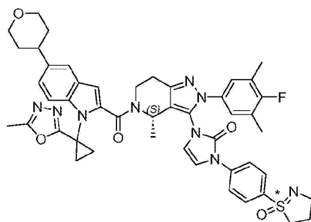
Compound 156
