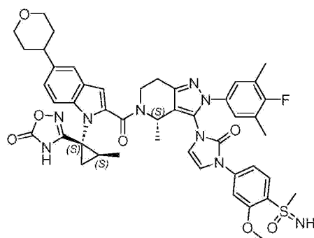
Compound 123
