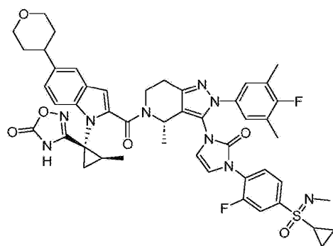
Compound 221
