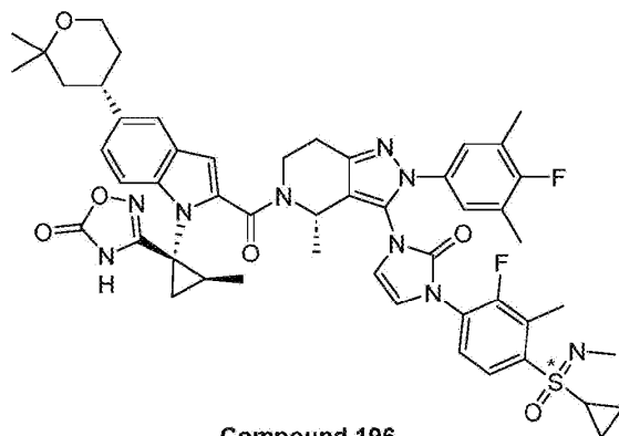
Compound 196
