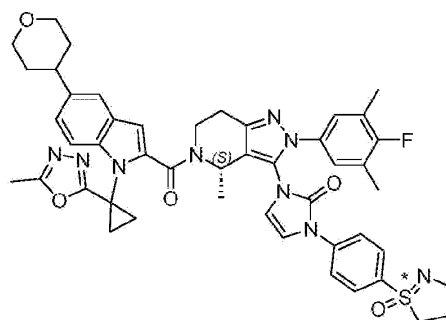
Compound 155
