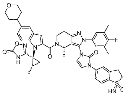
Compound 101
