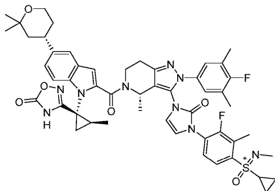
Compound 195
