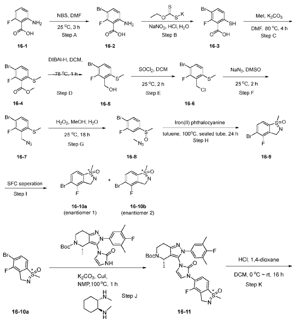
Compound 187
