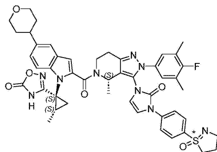
Compound 142 enantiomer 1
