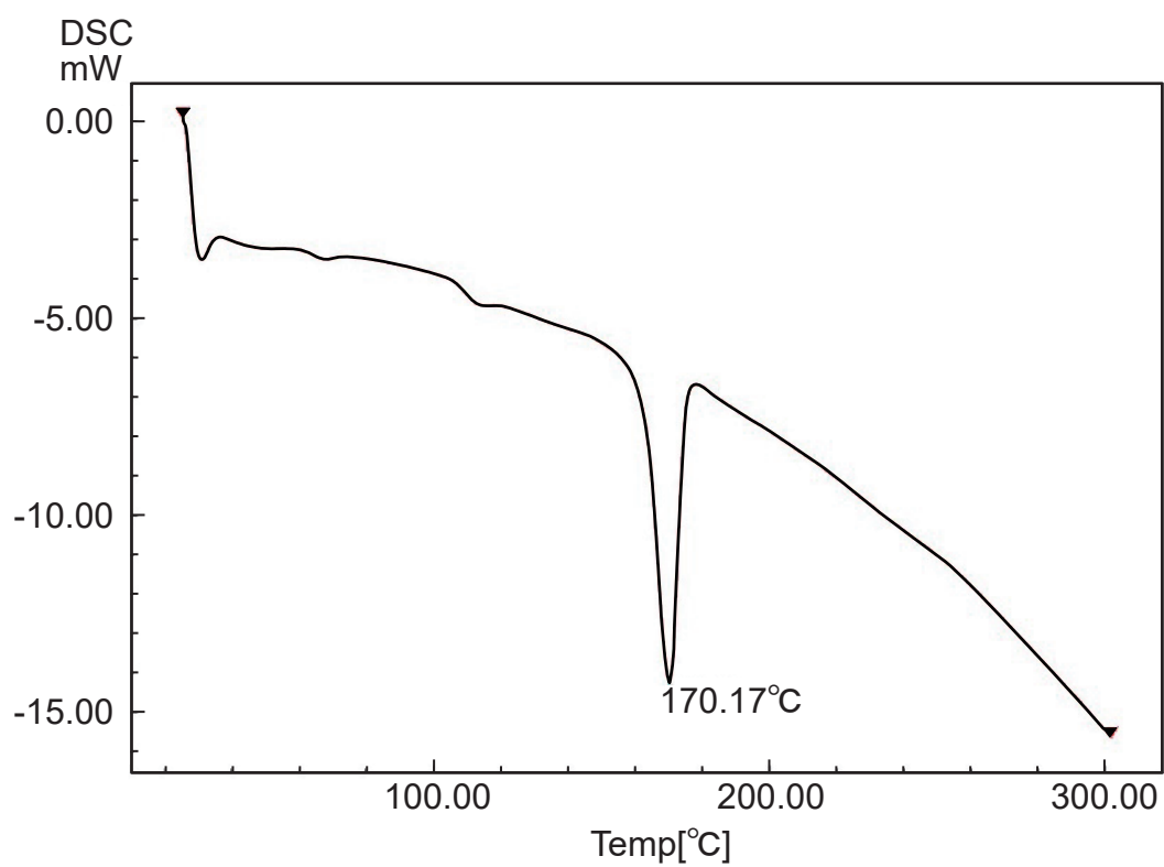
Resin particle (c4) DSC peak at 170°C
