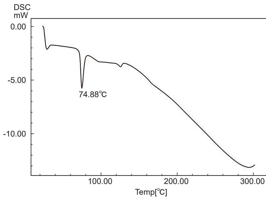
Resin particle (c11) DSC peak 75°C
