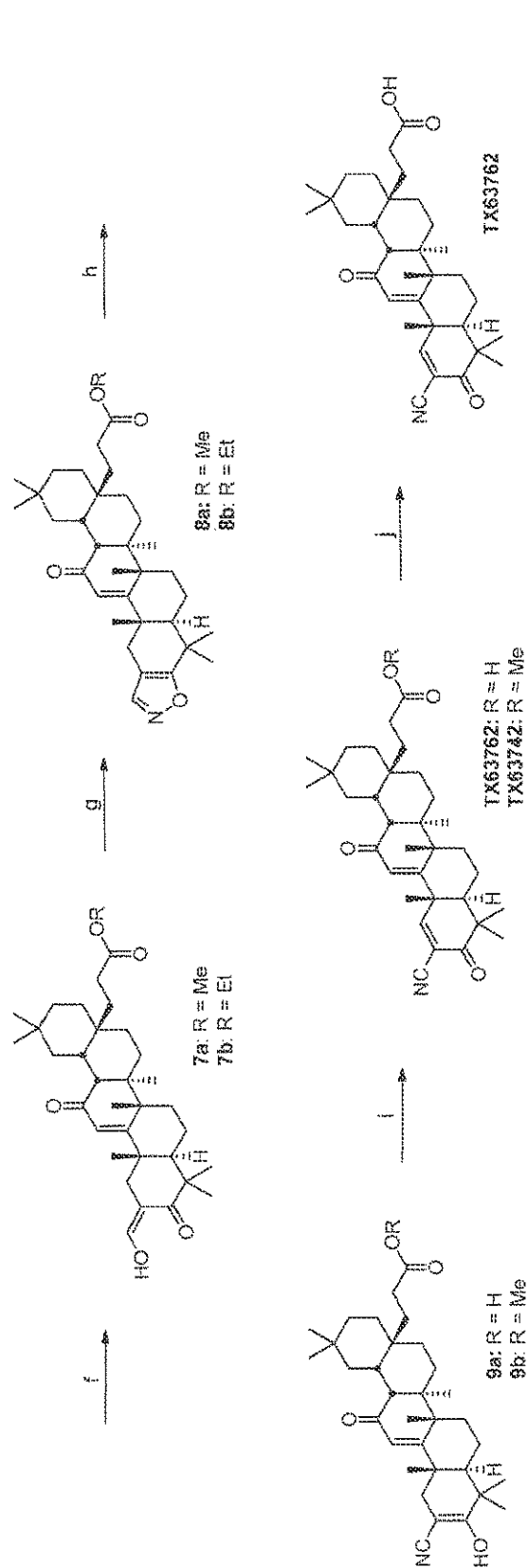
Scheme 1b
