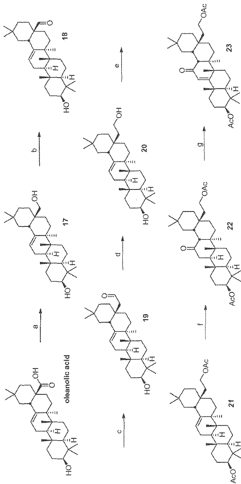
Scheme 12a
