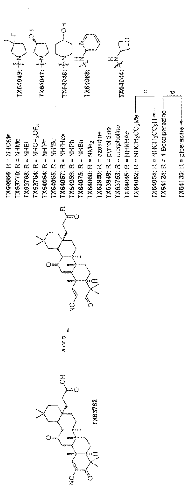
Scheme 5
