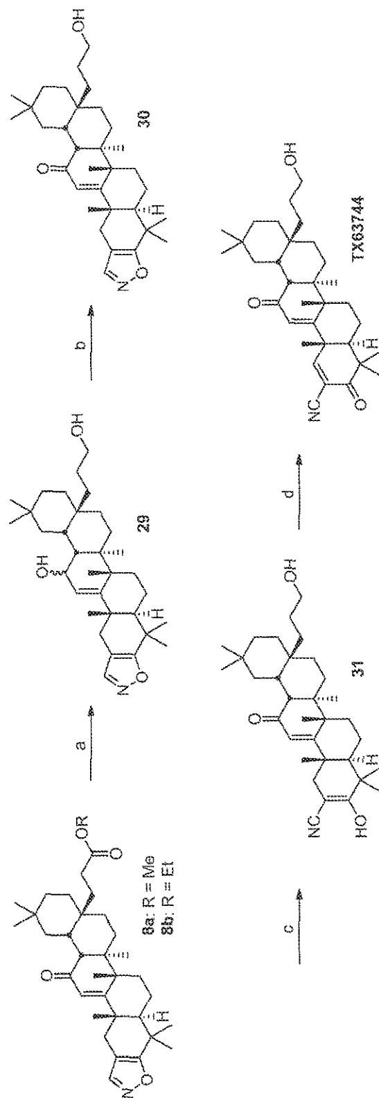
Scheme 15
