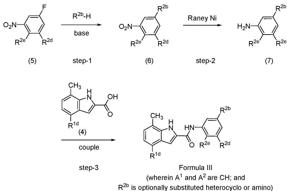
General Scheme 2
