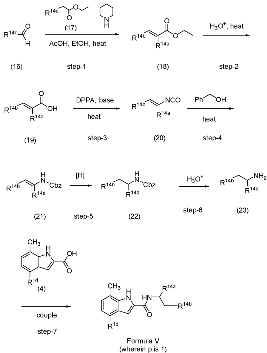
General Scheme 6
