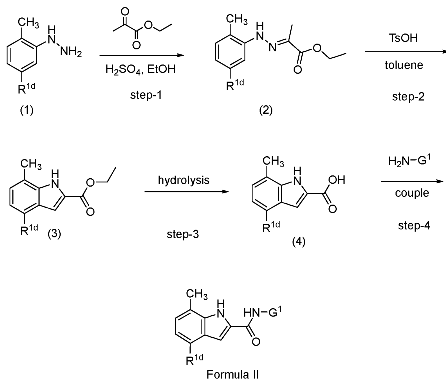
General Scheme 1
