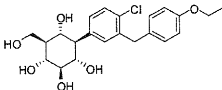
(1 R ,2 R ,3 S ,4 R ,5 R ,6 S )-4-(4-chloro-3-(4-ethoxybenzyl)phenyl)-6-(hydroxymethyl)cyclohexane-1,2,3,5-tetraol
