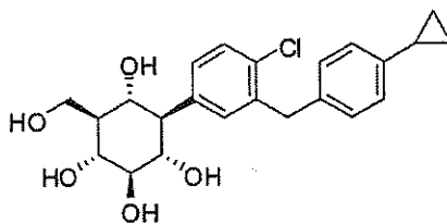
(1 R ,2 R ,3 S ,4 R ,5 R ,6 S )-4-(4-chloro-3-(4-cyclopropylbenzyl)phenyl)-6-(hydroxymethyl)cyclohexane-1,2,3,5-tetraol
