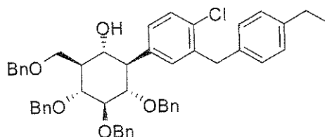
4 (R = Et)
