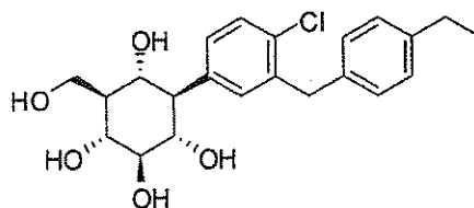
(1 R ,2 R ,3 S ,4 R ,5 R ,6 S )-4-(4-chloro-3-(4-ethylbenzyl)phenyl)-6-(hydroxymethyl)cyclohexane-1,2,3,5-tetraol
