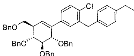
3 (R = Et)
