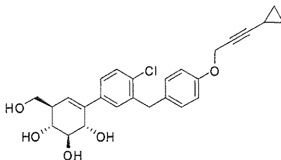
(1R,2S,3S,6R)-4-(4-chloro-3-(4-(3-cyclopropylprop-2-ynyloxy)benzyl)phenyl)-6-(hydroxymethyl)cyclohex-4-ene-1,2,3-triol
