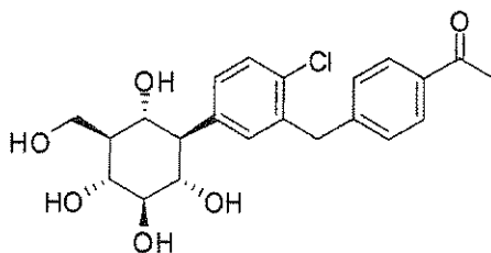
1-(4-(2-chloro-5-((1R,2S,3R,4R,5S,6R)-2,3,4,6-tetrahydroxy-5-(hydroxymethyl)cyclohexyl)benzyl)phenyl)ethanone
