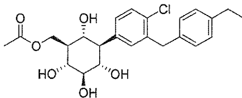
((1S,2R,3R,4S,5R,6R)-3-(4-chloro-3-(4-ethylbenzyl)phenyl)-2,4,5,6-tetrahydroxycyclohexyl)methyl acetate
