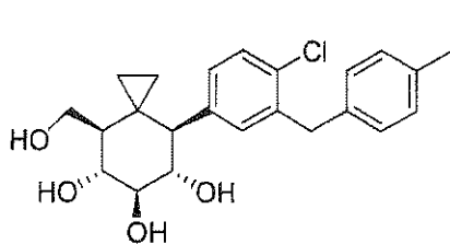
(4S,5S,6R,7R,8R)-4-(4-chloro-3-(4-ethylbenzyl)phenyl)-8-(hydroxymethyl)spiro[2.5]octane-5,6,7-triol
