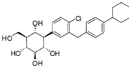
(1R,2R,3S,4R,5R,6S)-4-(4-chloro-3-(4-cyclohexylbenzyl)phenyl)-6-(hydroxymethyl)cyclohexane-1,2,3,5-tetraol
