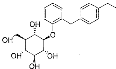
(1R,2S,3R,4R,5S,6R)-4-(2-(4-ethylbenzyl)phenoxy)-6-(hydroxymethyl)cyclohexane-1,2,3,5-tetraol
