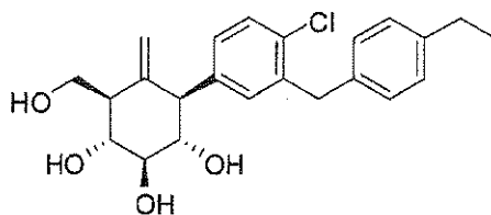
(1R,2R,3S,4S,6R)-4-(4-chloro-3-(4-ethylbenzyl)phenyl)-6-(hydroxymethyl)-5-methylenecyclohexane-1,2,3-triol
