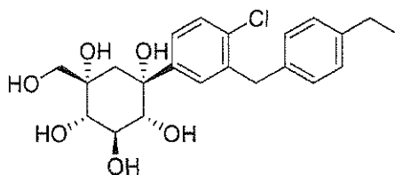
22 (R = Et)
