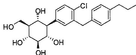
(1 R ,2 R ,3 S ,4 R ,5 R ,6 S )-4-(4-chloro-3-(4-propylbenzyl)phenyl)-6-(hydroxymethyl)cyclohexane-1,2,3,5-tetraol
