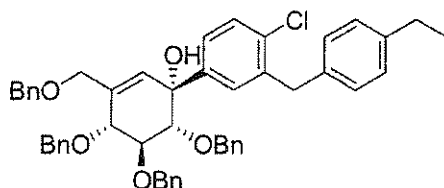
2 (R = Et)
