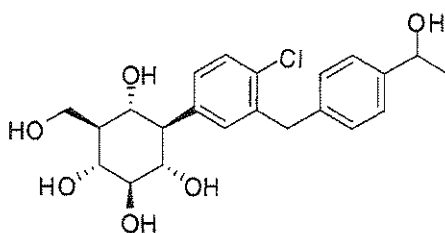
(1R,2R,3S,4R,5R,6S)-4-(4-chloro-3-(4-(1-hydroxyethyl)benzyl)phenyl)-6-(hydroxymethyl)cyclohexane-1,2,3,5-tetraol
