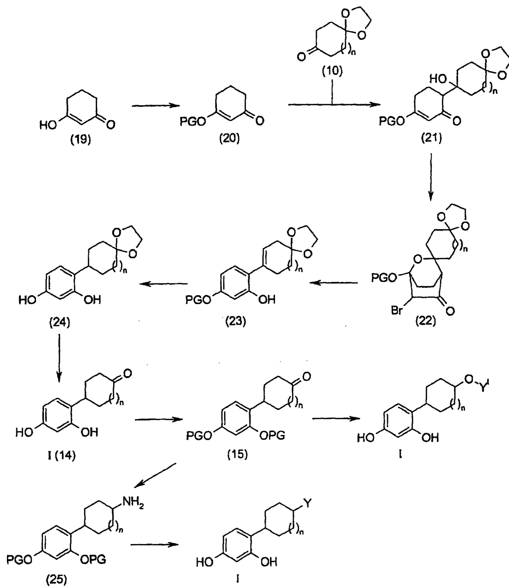
Scheme 3
