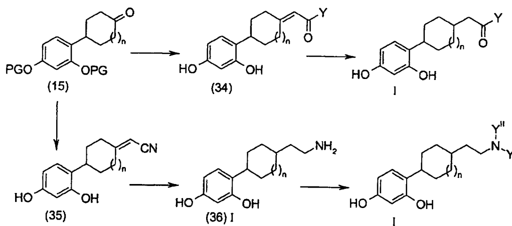
Scheme 9
