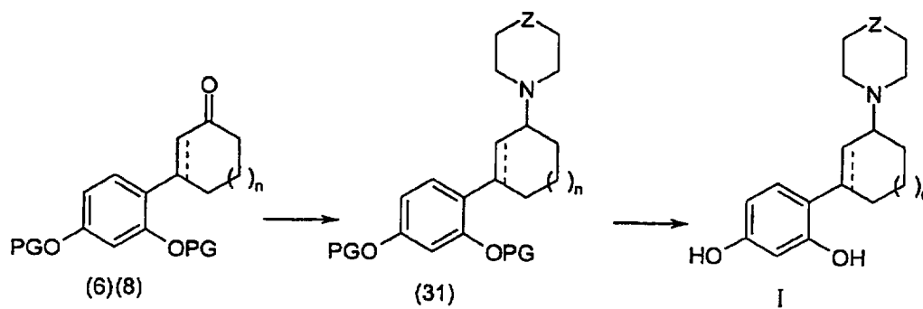
Scheme 7
