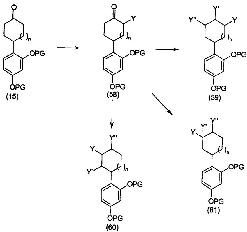
Scheme 12
