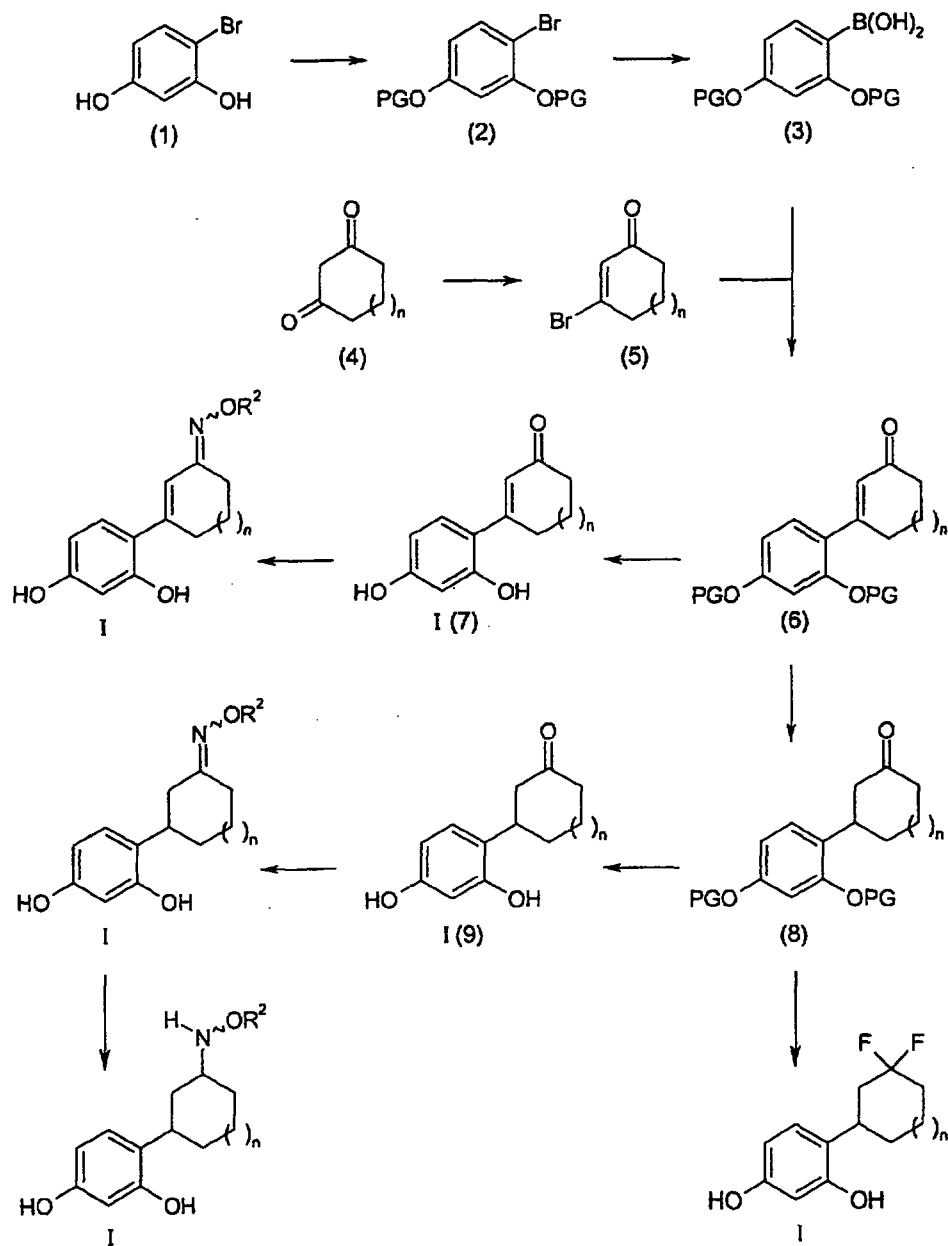
Scheme 1
