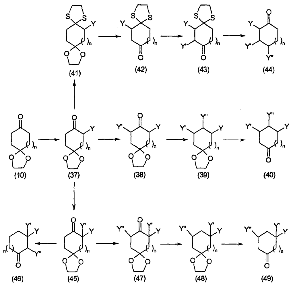
Scheme 10
