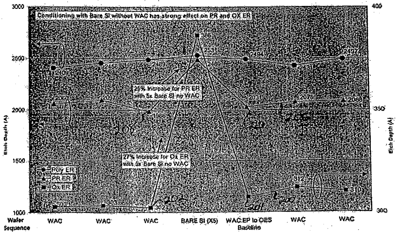
Figure 10. Effect of WAC on Etchrate Performance
