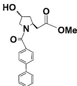
(16b)
