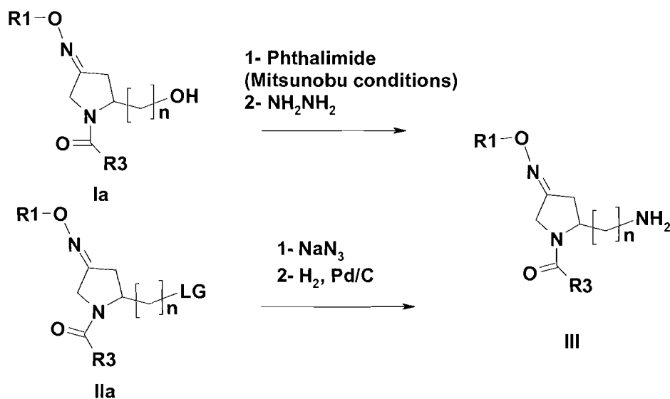
Scheme 13:
