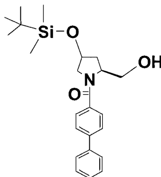
(15b)
