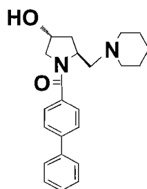
(15d)
