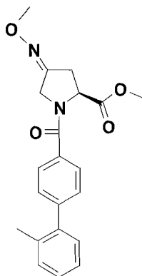
(1d)
