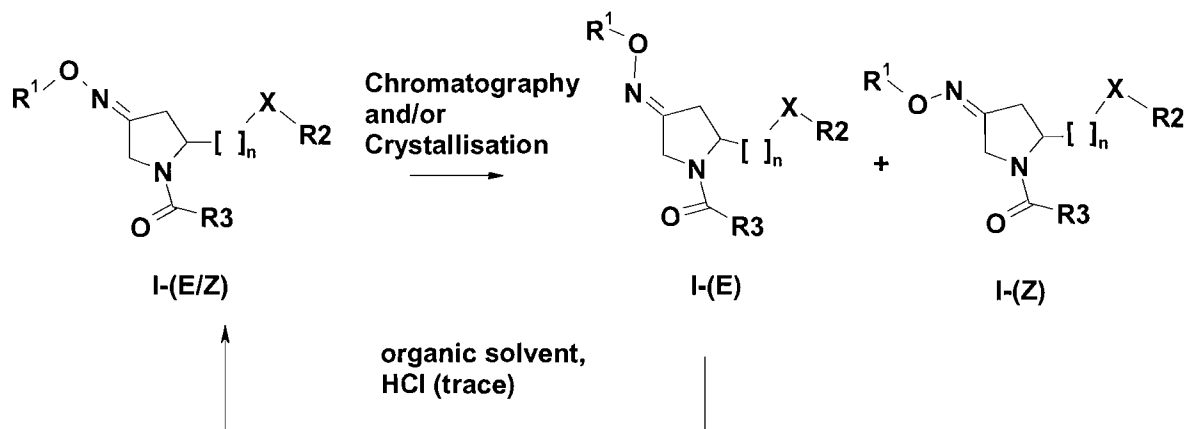
Scheme 18:
