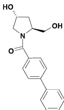
( 2b )
