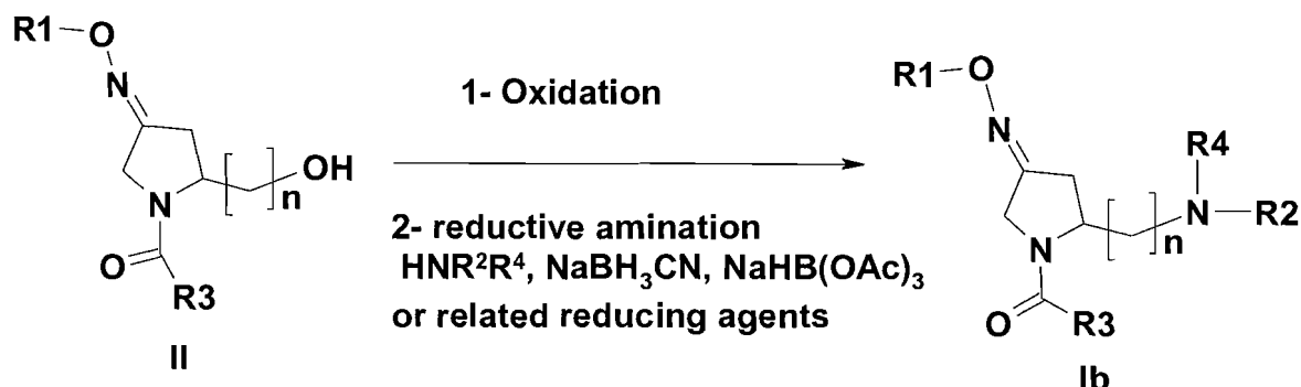
Scheme 11:
