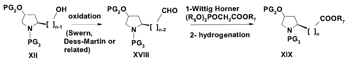
Scheme 9:
