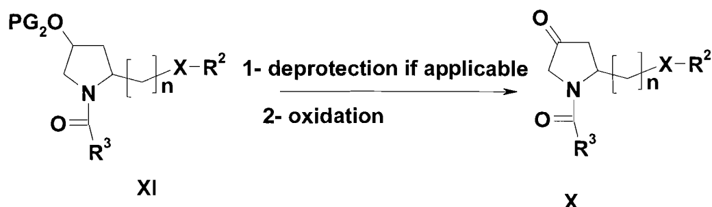
Scheme 16:
