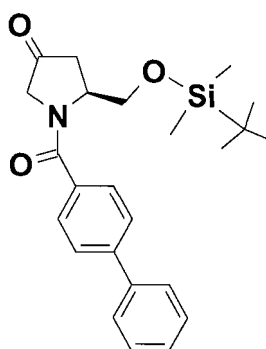
(2d)
