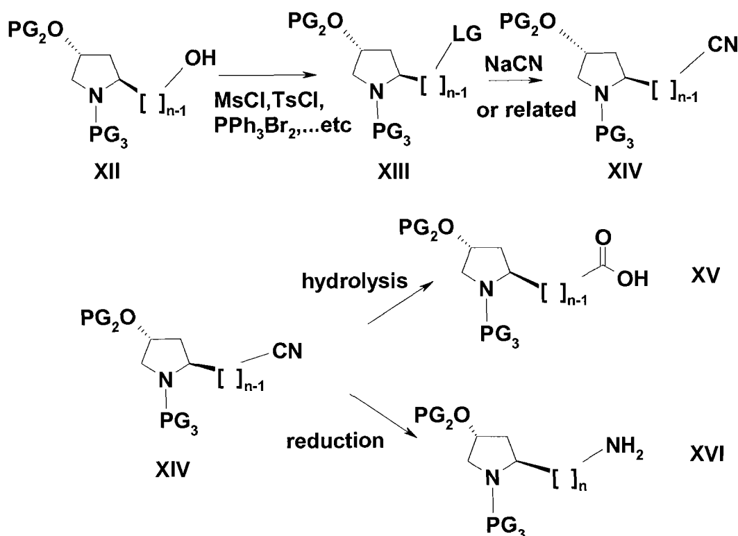
Scheme 8:
