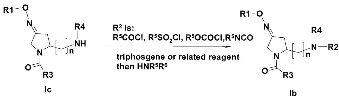
Scheme 14:
