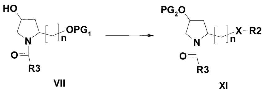
Scheme 17:
