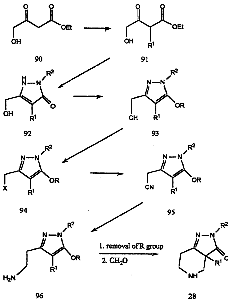
SCHEME 25: Treatment of a hydroxyacetoacetate ester of formula 90 with an alkyl halide in the presence of a suitable base such as sodium hydride affords compounds of formula 91. Reaction of 91 with a hydrazine generates compounds of formula 92. O-Alkylation of the carbonyl oxygen of 92 affords 93 which is converted to the halide 94. Displacement of the halide X by cyanide ion affords
