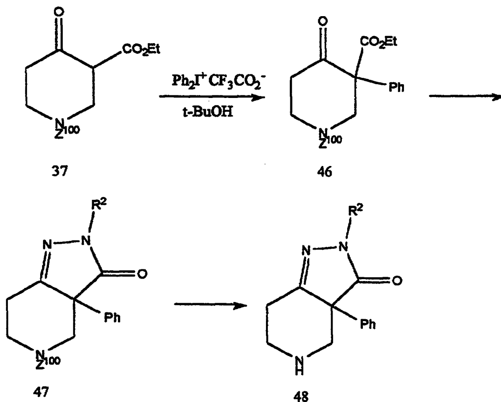
Scheme 13: Treatment of a ketoester of formula 37 with an iodonium salt such as diphenyliodonium trifluoroacetate in a suitable solvent such as t-butanol generates a ketoester of formula 46. Reaction of 46 with a hydrazine generates a compound of formula 47. Deprotection of the nitrogen affords compounds of formula 48, see Synthesis, (9), 1984 p. 709 for a detailed description.
