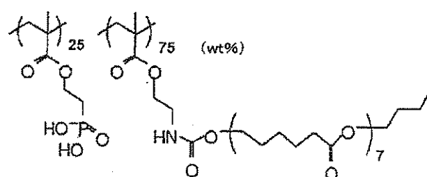
(Exemplary Compound 12) Acid value 144mgKOH/g
