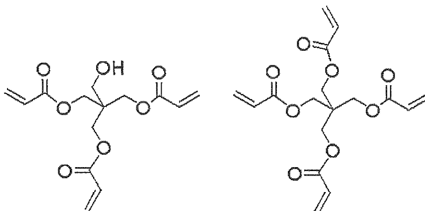
Polymerizable Compound 6 (The molar ratio of the left compound and the right compound = 6:4)
