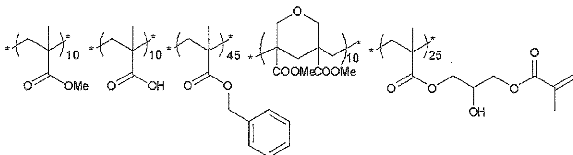
Alkali-Soluble Resin 1 (the ratio in the repeating unit is a molar ratio)
