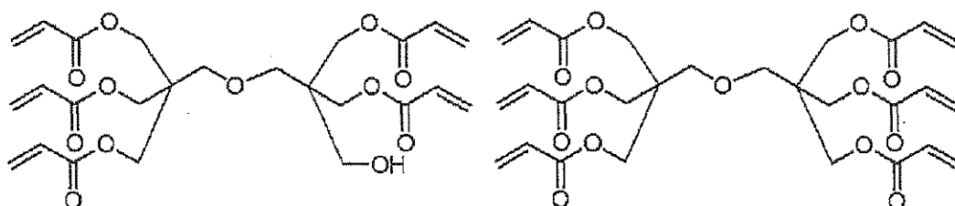
Polymerizable Compound 1 (A mixture of the left compound and the right compound with a molar ratio of 7:3)
