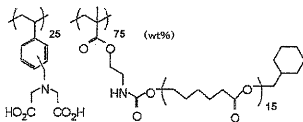
(Exemplary Compound 13) Acid value 113mgKOH/g
