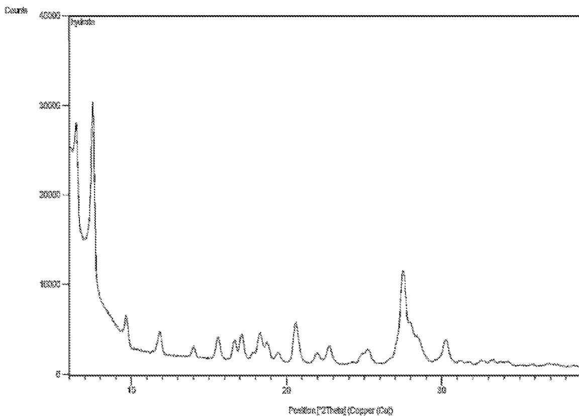
FIGURE 1b: XRPD Compound I-1 (hydrate)
