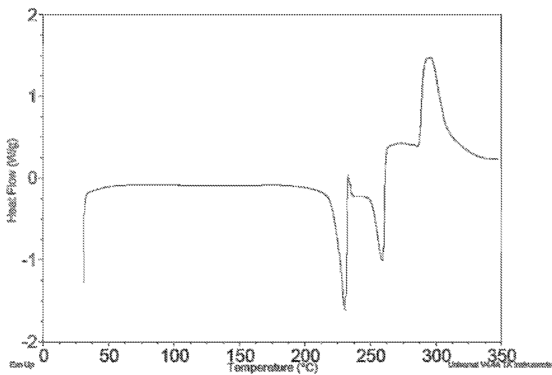
FIGURE 3c: DSC Compound I-1 (tartaric acid)
