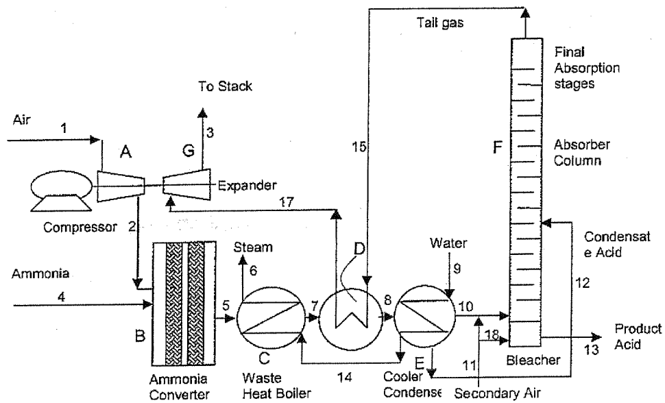
Figure 1. Nitric Acid production process
