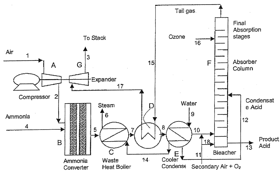
Figure 3. Nitric Acid production process retrofitted with Ozone oxidation and O 2 enrichment
