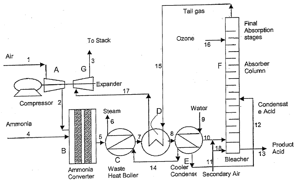
Figure 2. Nitric Acid production process retrofitted with Ozone oxidation
