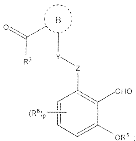
IIIA
