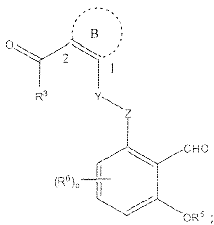
IIIC
