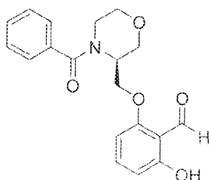
(S)-2-((4-benzoylmorpholin-3-yl)methoxy)-6-hydroxybenzaldehyde
