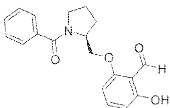
(S)-2-((1-benzoylpyrrolidin-2-yl)methoxy)-6-hydroxybenzaldehyde
