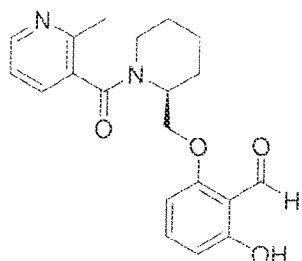
(S)-2-hydroxy-6-((1-(2-methylnicotinoyl)piperidin-2-yl)methoxy)benzaldehyde
