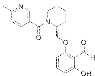
(S)-2-hydroxy-6-((1-(6-methylnicotinoyl)piperidin-2-yl)methoxy)benzaldehyde
