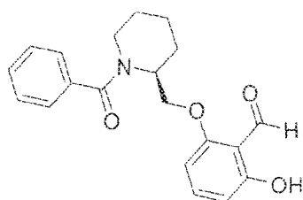
(S)-2-((1-benzoylpiperidin-2-yl)methoxy)-6-hydroxybenzaldehyde
