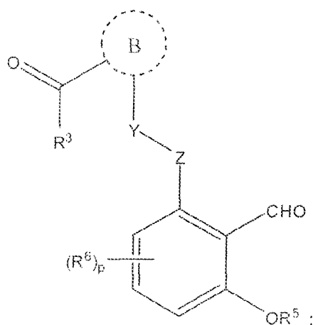
IIIA
