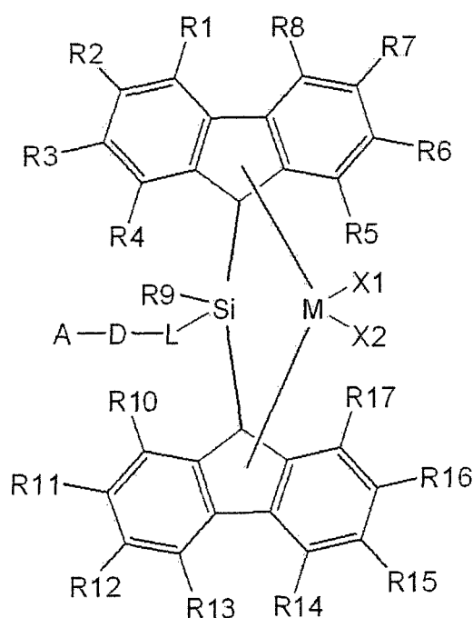
[Chemical Formula 1]
