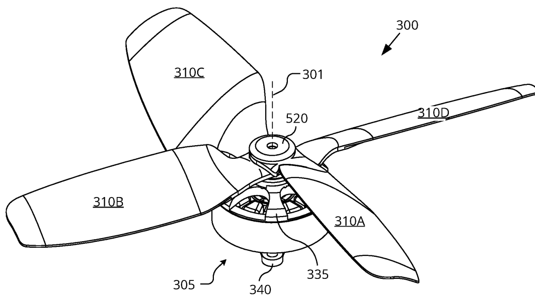
DEPLOYED POSITION (UNFOLDED PROPELLER BLADES)
