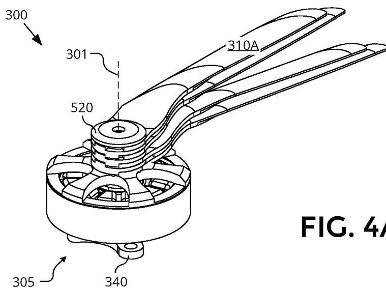
STOWED POSITION (FOLDED PROPELLER BLADES)
