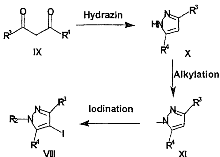
Scheme 4
