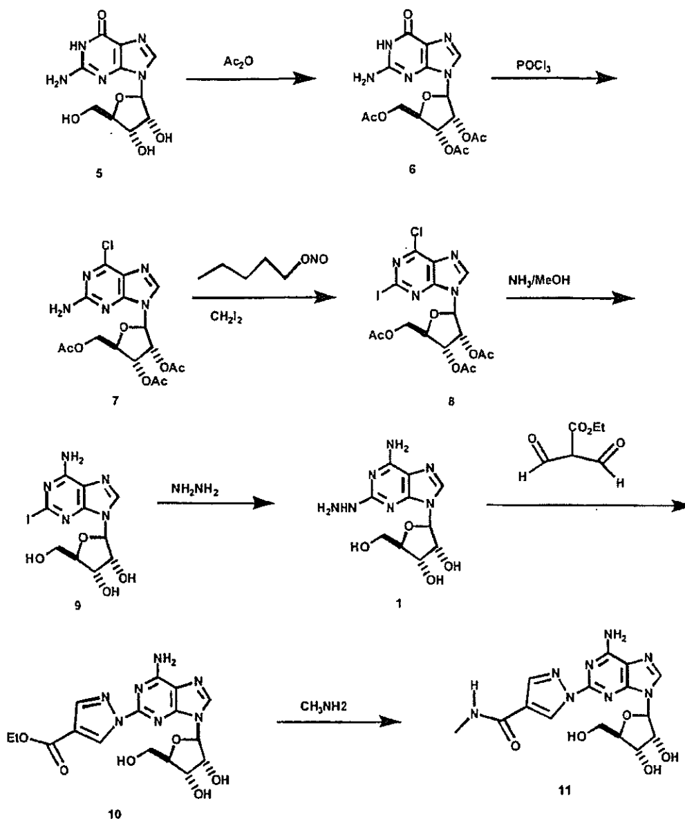
Scheme 3
