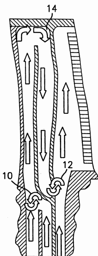
FIG. 1 (PRIOR ART)
