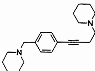
1-[4-(4-Piperidin-1-ylmethyl-phenyl)-but-3-ynyl]-piperidine
