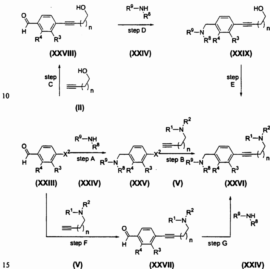
Scheme 5
