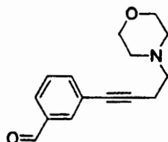
3-(4-Morpholin-4-yl-but-1-ynyl)-benzaldehyde
