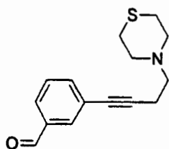
3-(4-Thiomorpholin-4-yl-but-1-ynyl)-benzaldehyde
