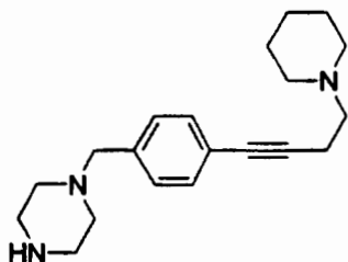
1-[4-(4-Piperidin-1-yl-but-1-ynyl)-benzyl]-piperazine
