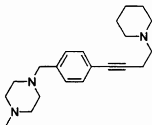
1-Methyl-4-[4-(4-piperidin-1-yl-but-1-ynyl)-benzyl]-piperazine
