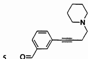
3-(4-Piperidin-1-yl-but-1-ynyl)-benzaldehyde
