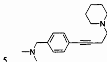
Dimethyl-[4-(4-piperidin-1-yl-but-1-ynyl)-benzyl]-amine
