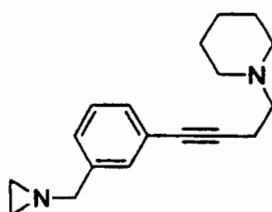
1-[4-(3-Aziridin-1-ylmethyl-phenyl)-but-3-ynyl]-piperidine
