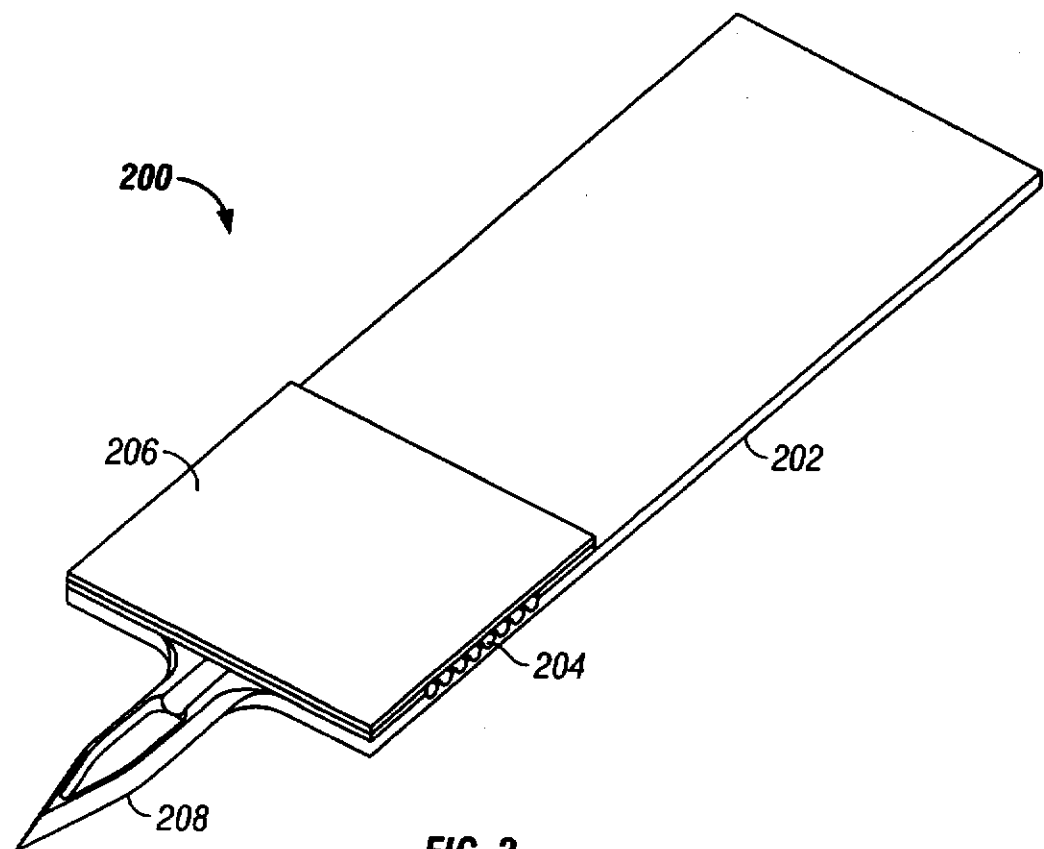
FIG. 2 (Prior Art)
