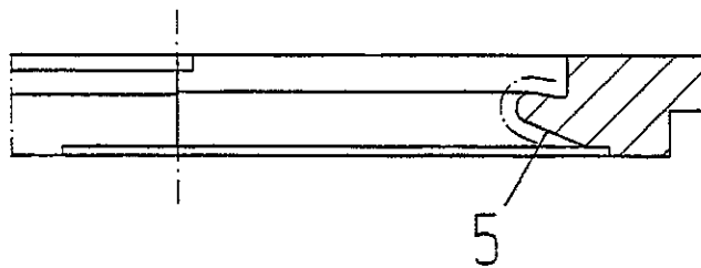
Detail Z
