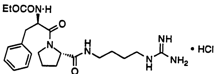
EtOCO-D-Phe-Pro-Agm·HCl
