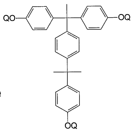
(XIII f)
