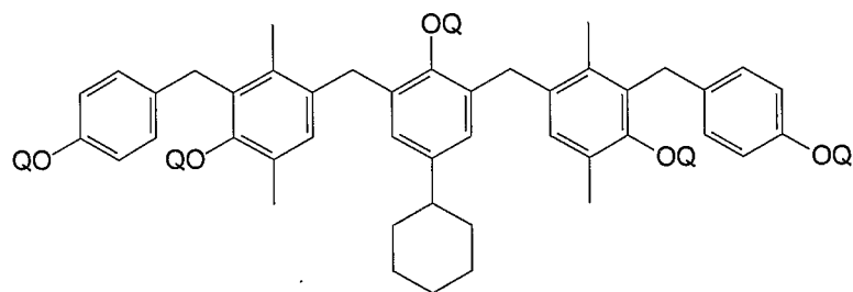
(XIII e)
