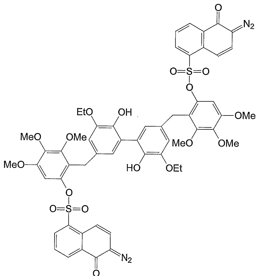
(XIIIq)
