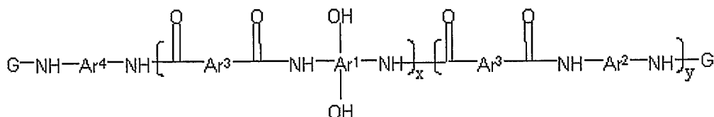
III
