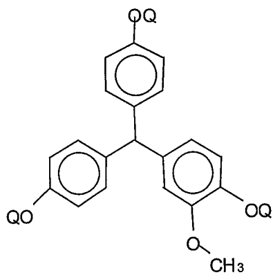
(XIII g)
