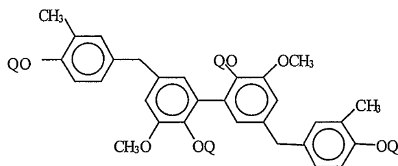
(XIII a)
