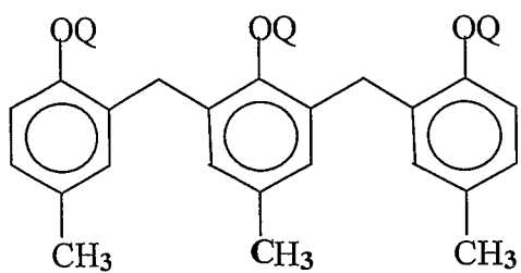
(XIII c)
