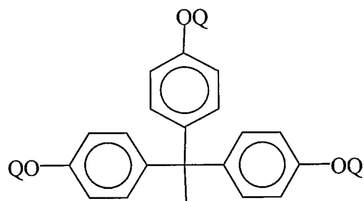
(XIII d)
