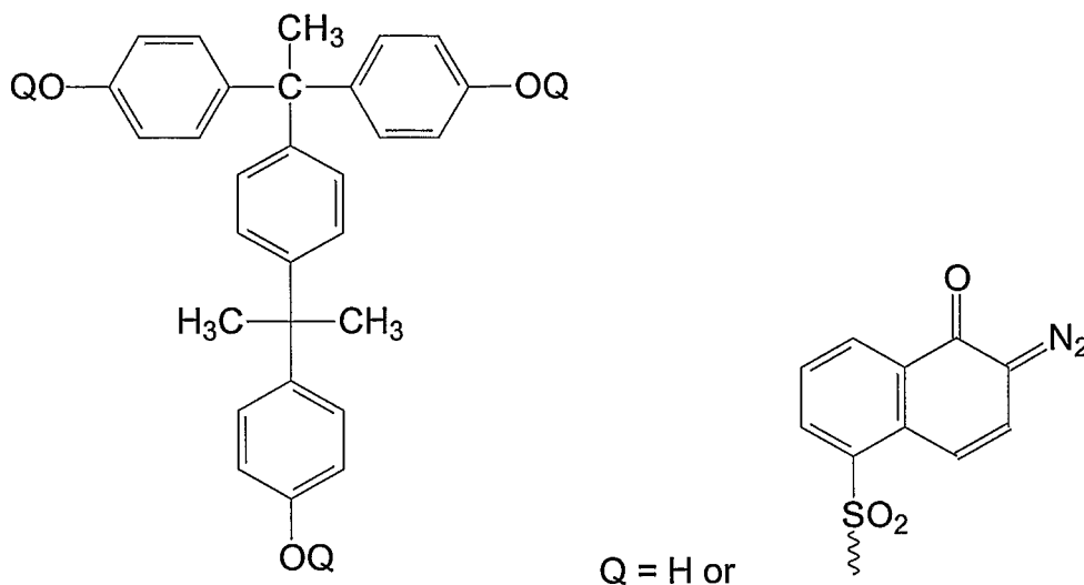
Structure of PAC XIII f (75% of OH groups are esterified)
