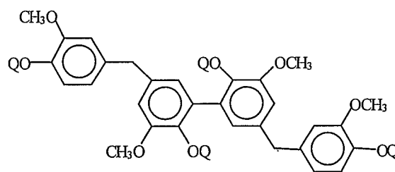
(XIII b)
