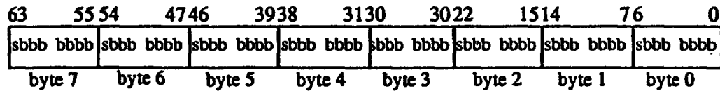
511 Signed Packed Byte In-Register Representation
