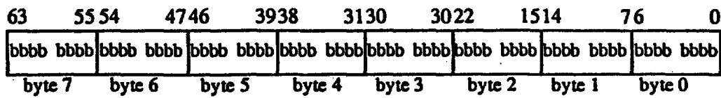
510 Unsigned Packed Byte In-Register Representation
