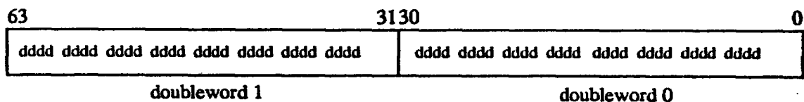
514 Unsigned Packed Doubleword In-Register Representation
