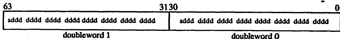
515 Signed Packed Doubleword In-Register Representation
