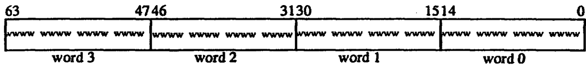
512 Unsigned Packed Word In-Register Representation
