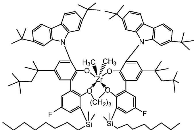
(8) ("Precatalyst 8");
