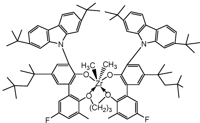
(6) ("Precatalyst 6")
