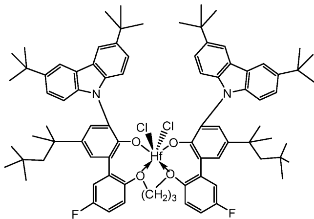
(7) ("Precatalyst 7")
