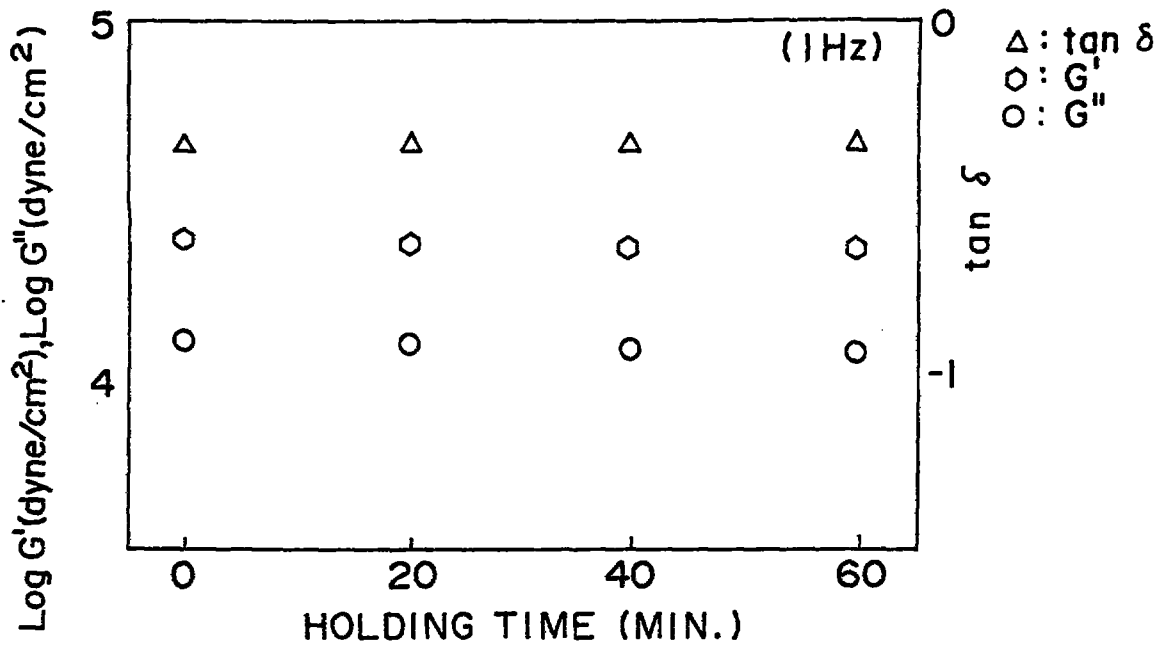
FIG. 3 (EXAMPLE 1 TONER, AT 1 Hz)
