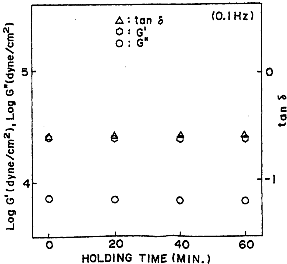
FIG. 8 (EXAMPLE 5 TONER, AT 0.1 Hz)
