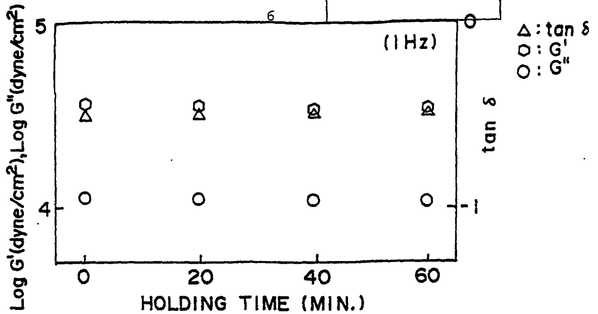
FIG. 7 (EXAMPLE 5 TONER, AT 1 Hz)
