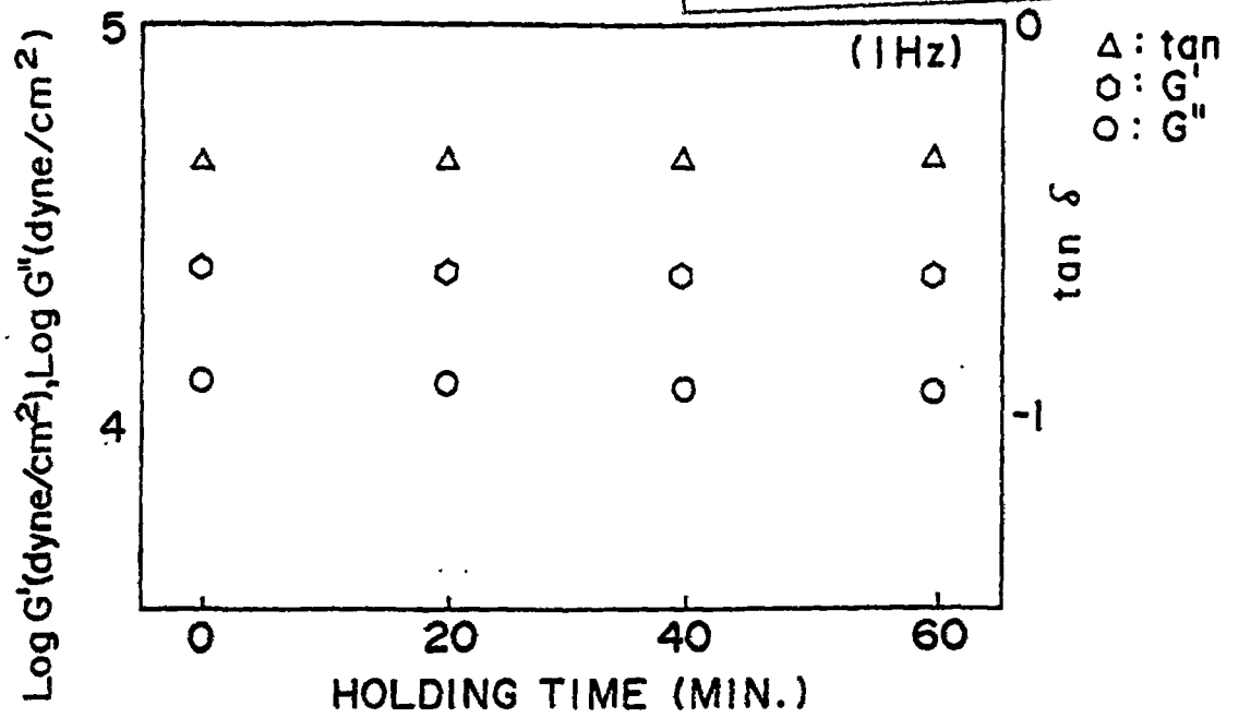
FIG. 3 (EXAMPLE 1 TONER, AT 1 Hz)
