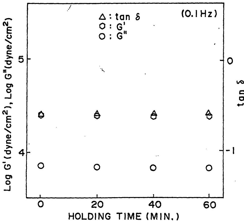
FIG. 8 (EXAMPLE 5 TONER, AT 0.1 Hz)
