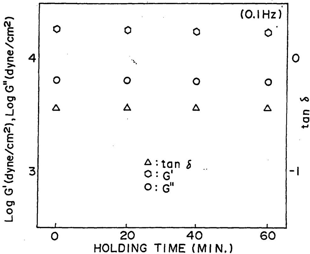
FIG. 4 (EXAMPLE 1 TONER, AT 0.1 Hz)
