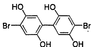
Compound U
