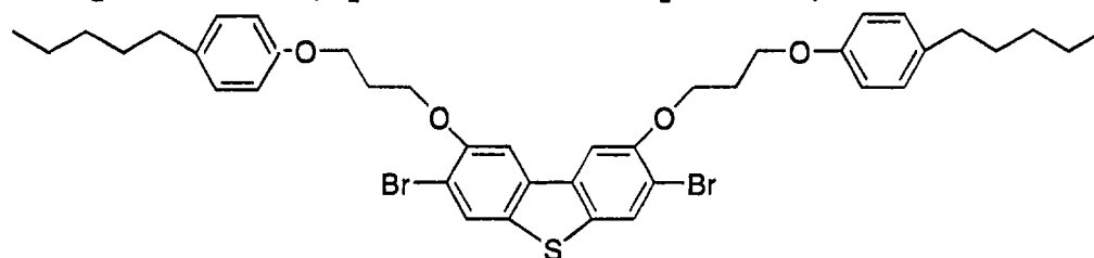
Compound J
