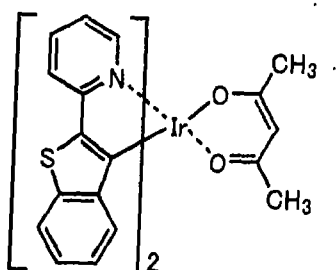
\text{Btp}_2\text{Ir(acac)}
