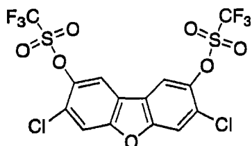
Compound S
