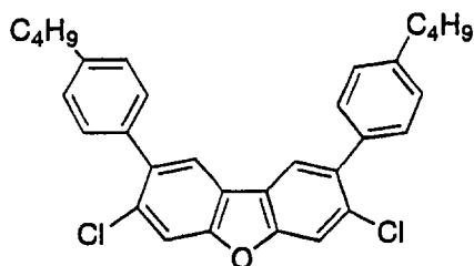
Compound T
