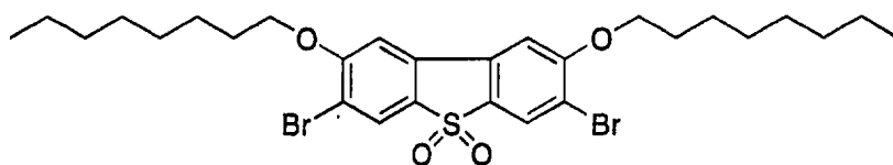
Compound D
