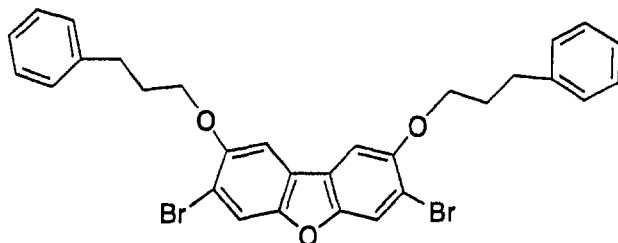
Compound X
