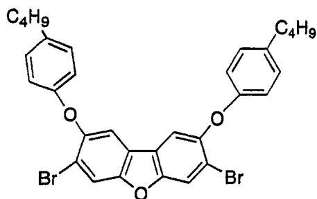
Compound W
