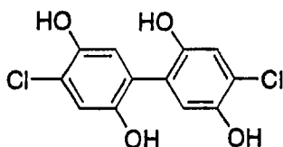
Compound Q
