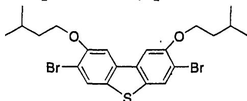
Compound G
