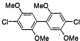
Compound P
