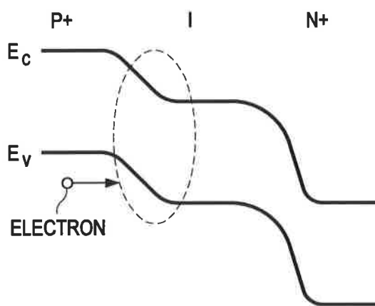
FIG. 1B OFF STATE TUNNELING IS NOT ALLOWED
