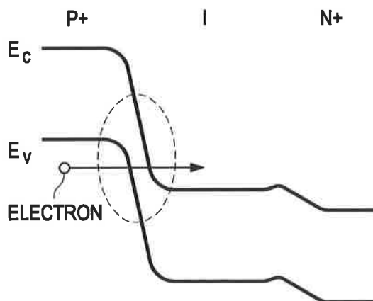
FIG. 1C ON STATE TUNNELING IS ALLOWED
