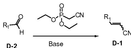
Scheme 9
