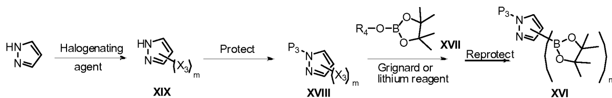
Scheme 14
