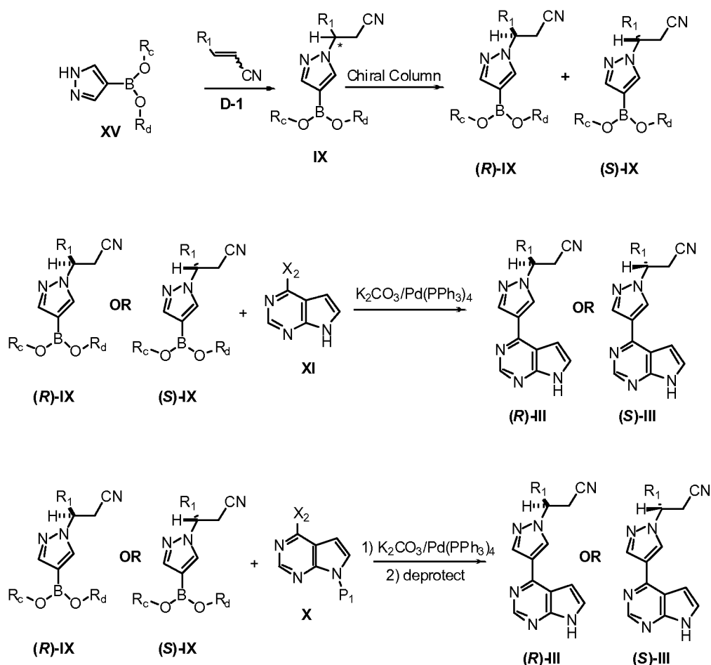
Scheme 5
