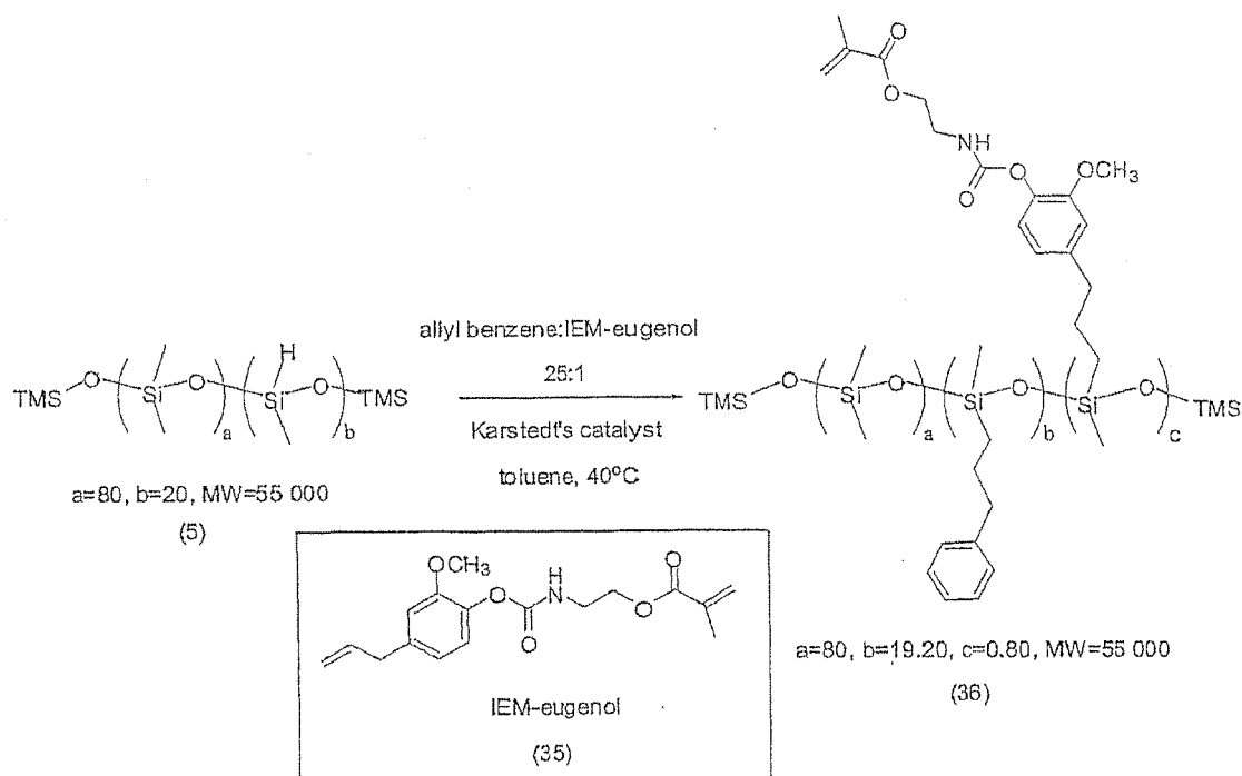
Scheme 7
