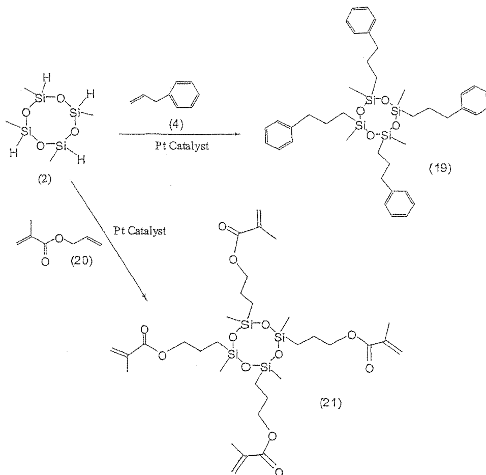
Scheme 9
