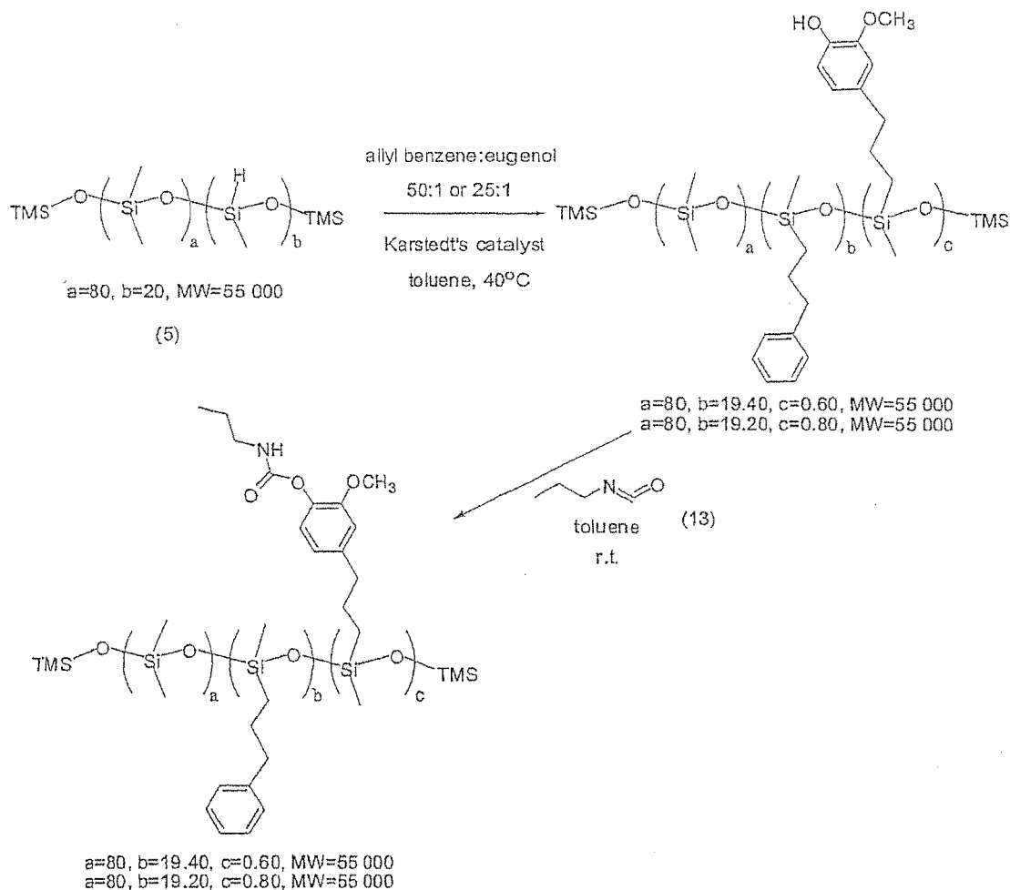
Scheme 6
