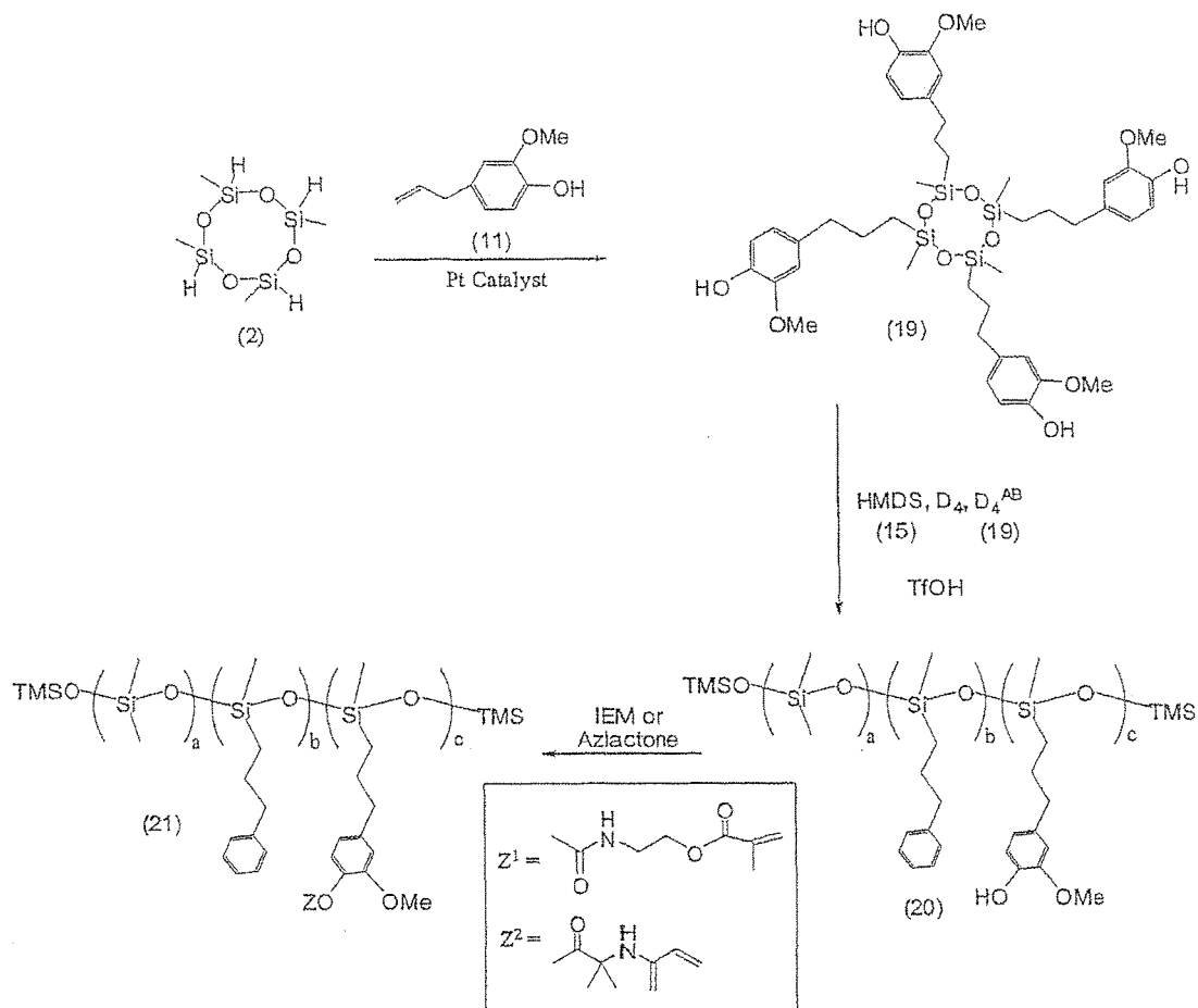
Scheme 8
