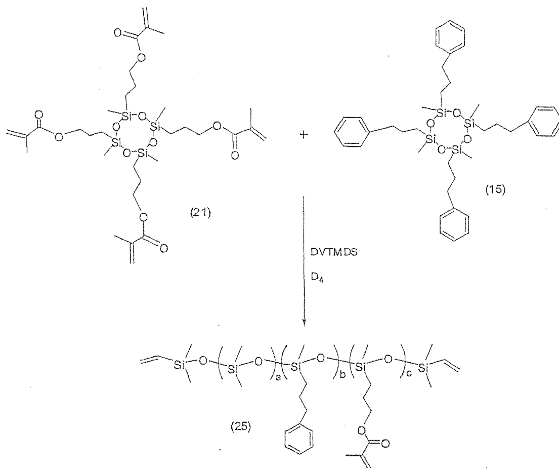
Scheme 11
