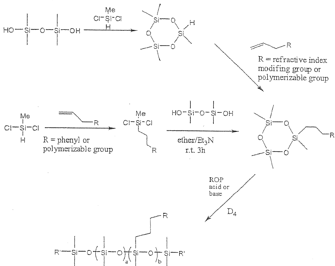
Scheme 14
