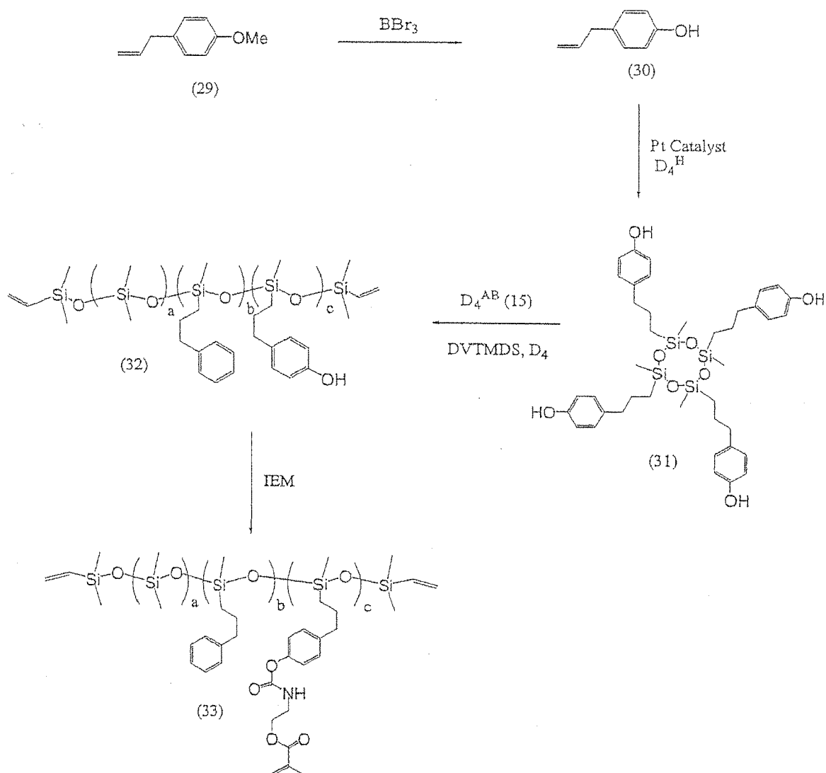
Scheme 13
