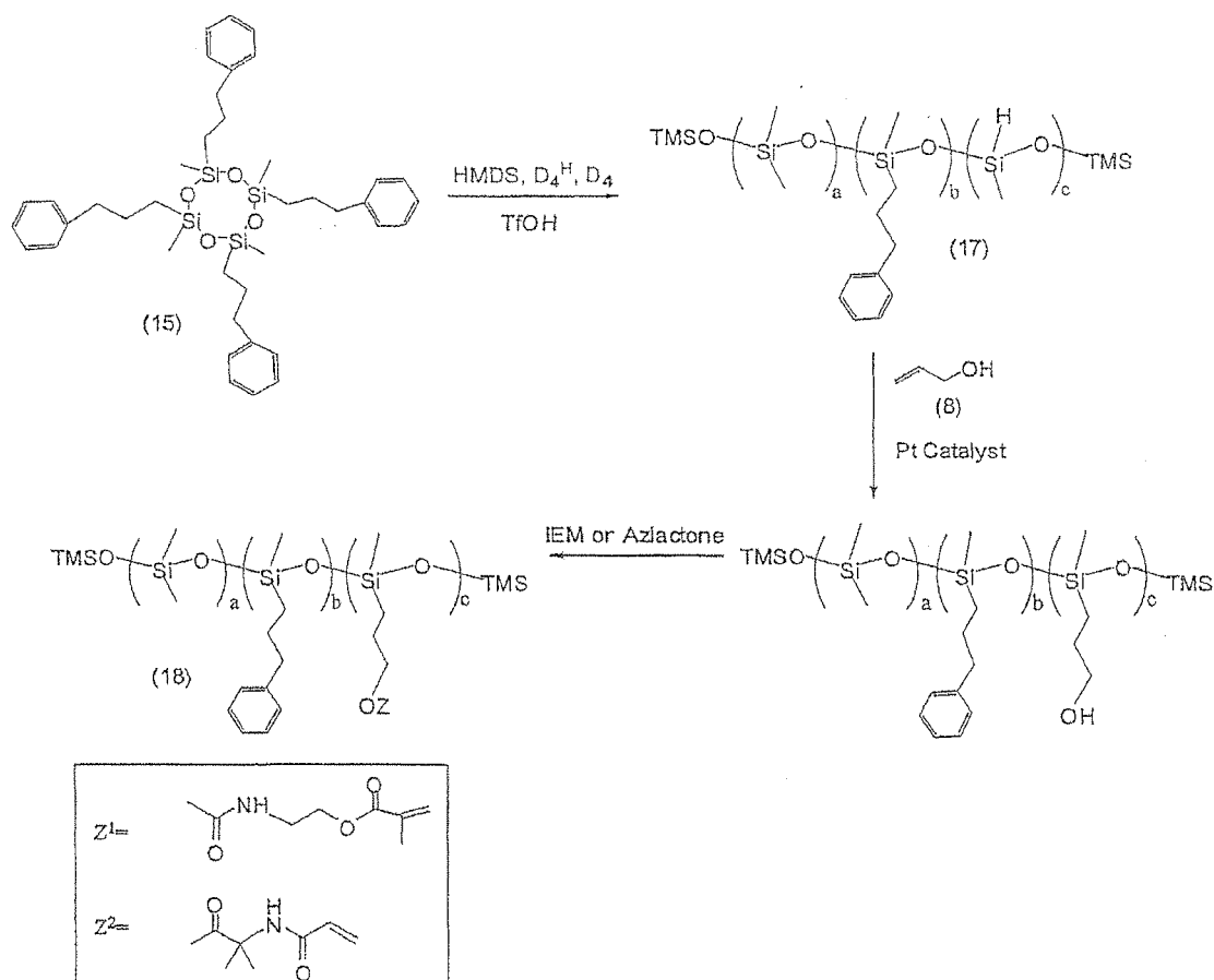
Scheme 10
