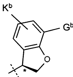
(S)-(Fb7)*
