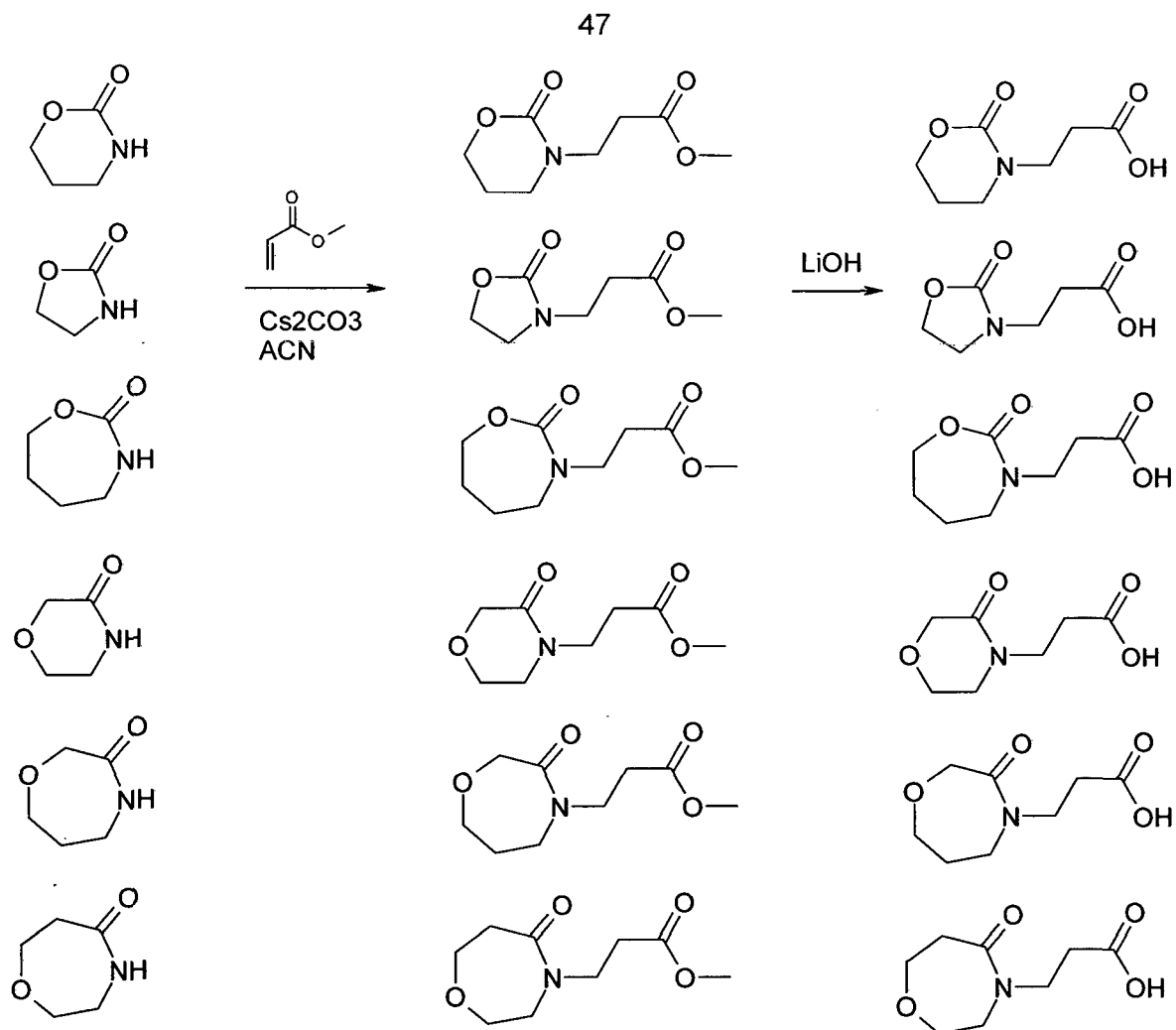
Scheme 7-1
