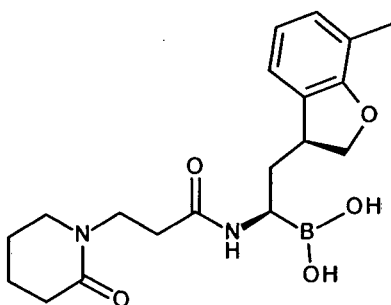
Compound No. 40: [(1R)-2-[(3S)-7-methyl-2,3-dihydrobenzofuran-3-yl]-1-[3-(2-oxo-1-piperidyl)propanoylamino]ethyl]boronic acid
