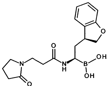
Compound No. 40: [(1R)-2-[(3S)-7-methyl-2,3-dihydrobenzofuran-3-yl]-1-[3-(2-oxo-1-piperidyl)propanoylamino]ethyl]boronic acid
