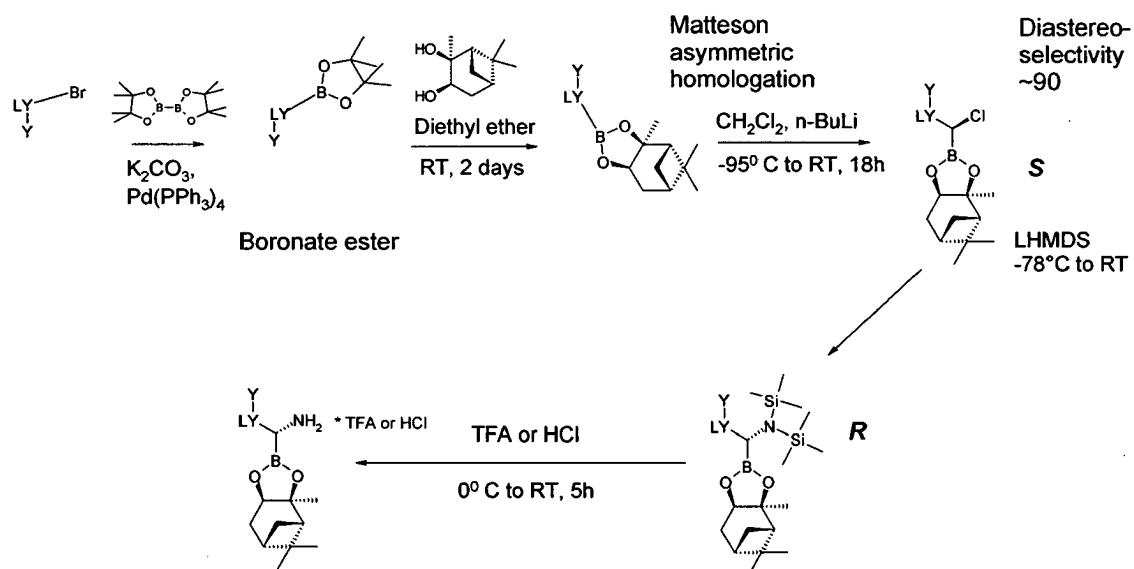
Scheme 3a
