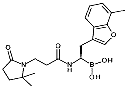
Compound No. 38: [(1R)-1-[3-(2,2-dimethyl-5-oxo-pyrrolidin-1-yl)propanoylamino]-2-(7-methylbenzofuran-3-yl)ethyl]boronic acid;
