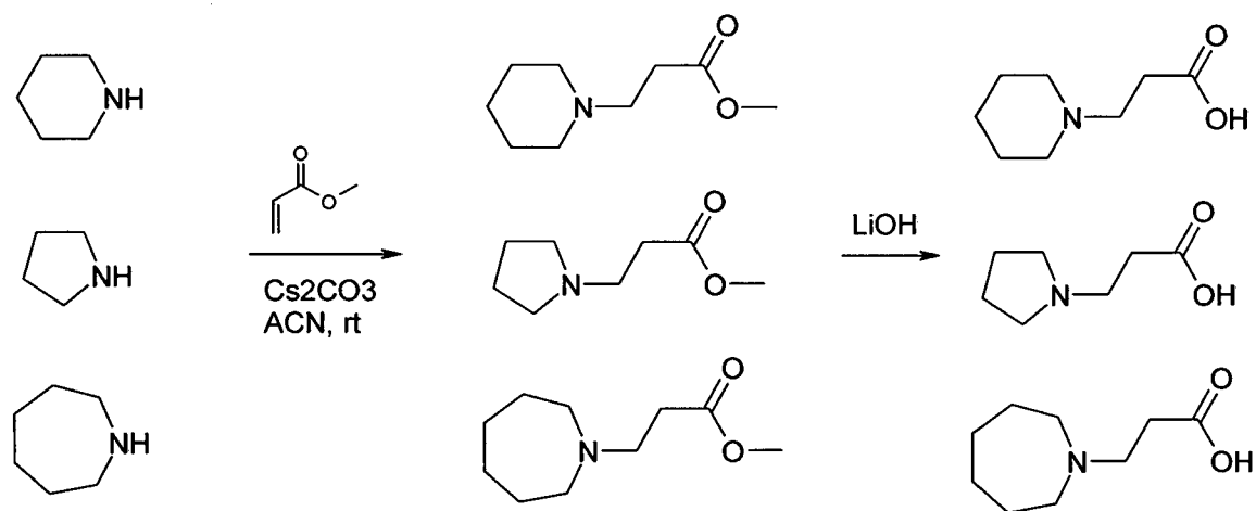
Scheme 5-1
