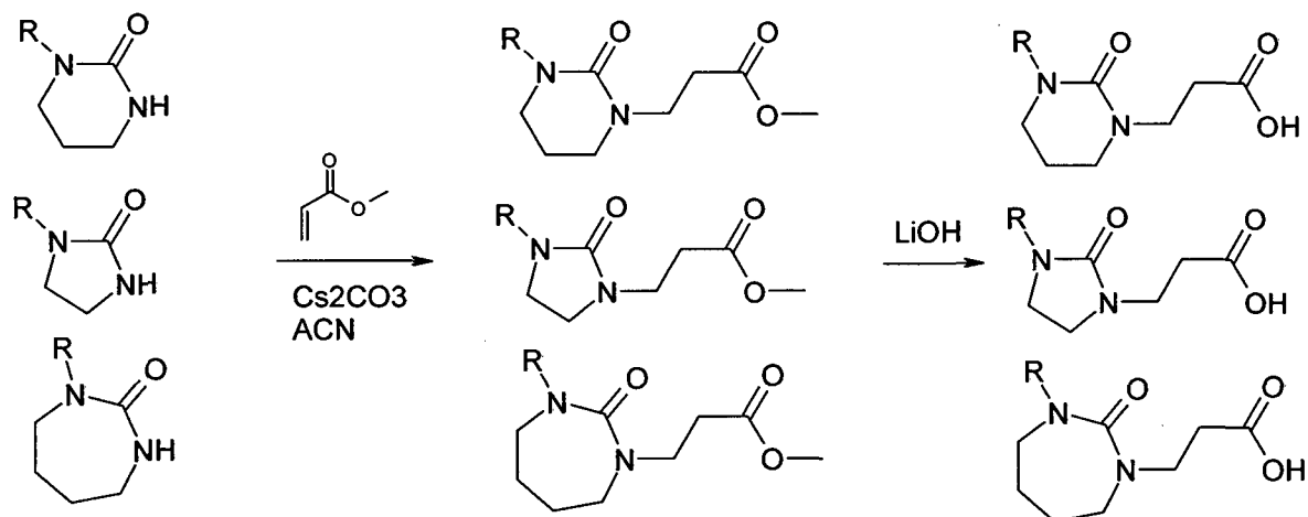
Scheme 7-1
