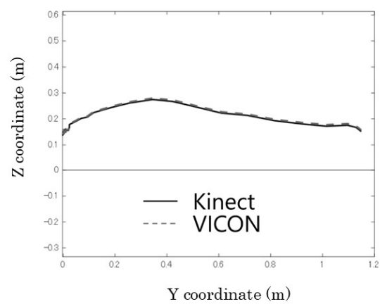
(B) Trajectory of right ankle while walking
