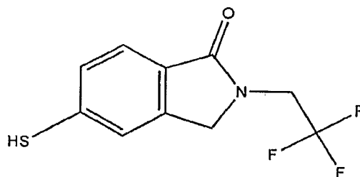
2-(2,2,2-trifluoroethyl)-5-mercaptoisoindolin-1-one
