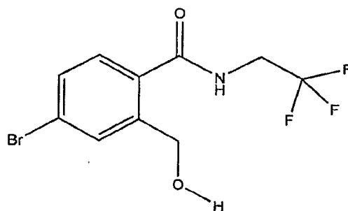
4-bromo-N-(2,2,2-trifluoroethyl)-2-(hydroxymethyl)benzamide
