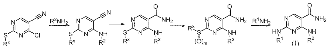
Scheme 5
