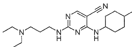
2-(3-(diethylamino)propylamino)-4-(4-methylcyclohexylamino)pyrimidine-5-carbonitrile
