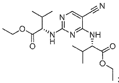
4-(cycloheptylamino)-2-(3-(2-methylpiperidin-1-yl)propylamino)-pyrimidine-5-carbonitrile
