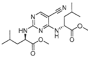
(2S,2'S)-diethyl 2,2'-(5-cyanopyrimidine-2,4-diyl)bis(azanediyl)-bis(3-methylbutanoate)
