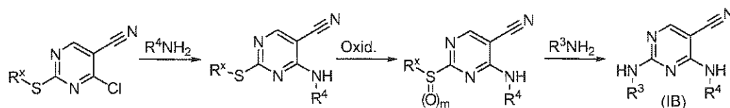
Scheme 9
