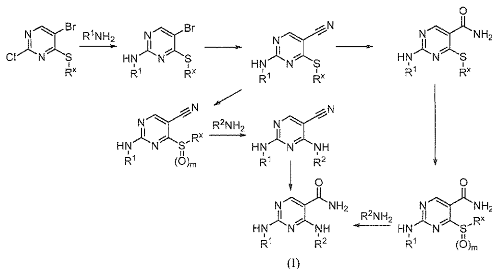
Scheme 6
