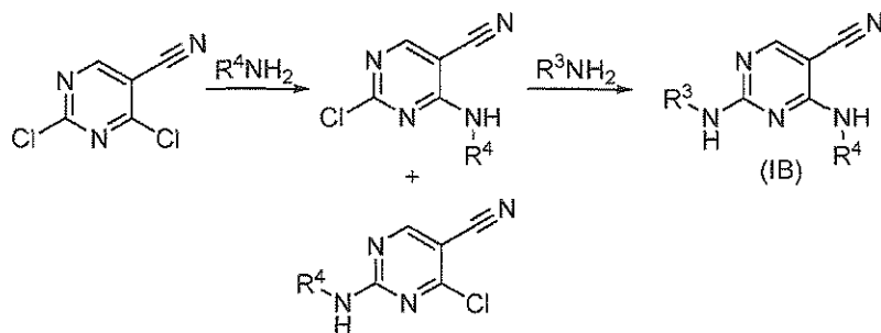
Scheme 7
