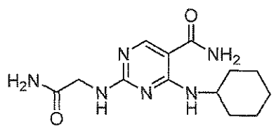
2-(2-aminoethylamino)-4-(cyclohexylamino)pyrimidine-5-carboxamide
