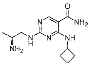
(S)-2-(2-aminopropylamino)-4-(cyclobutylamino)pyrimidine-5-carboxamide
