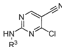
(VIa),
