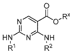
(IIIb),
