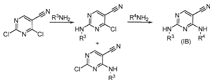
Scheme 8
