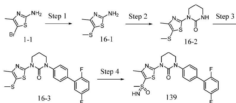
Scheme 16
