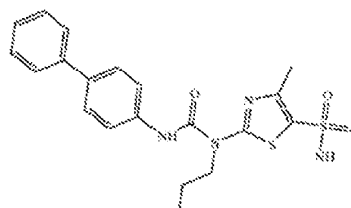
Example 152 WO200053591
