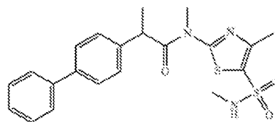
Example 45 WO2001047904
