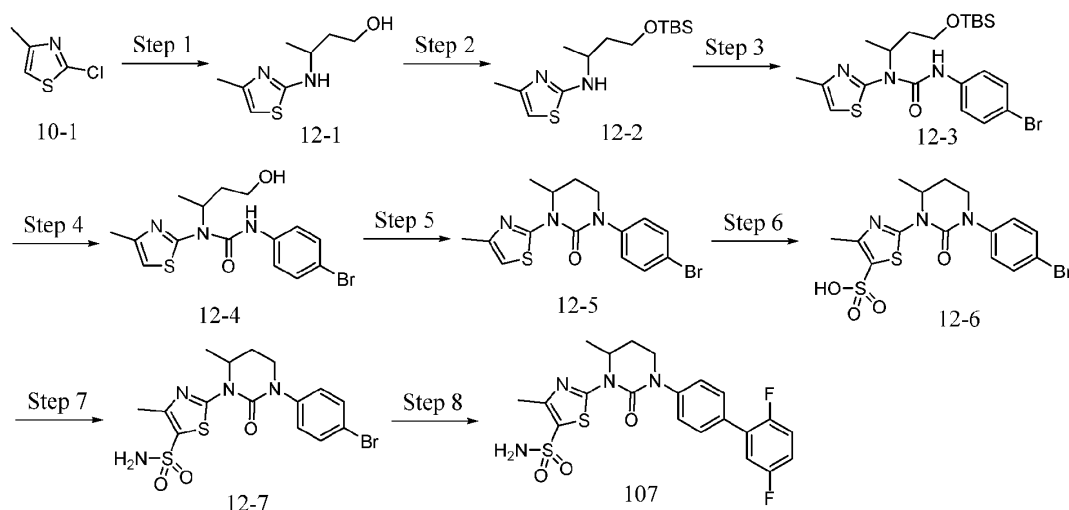
Scheme 12
