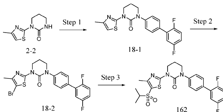
Scheme 18
