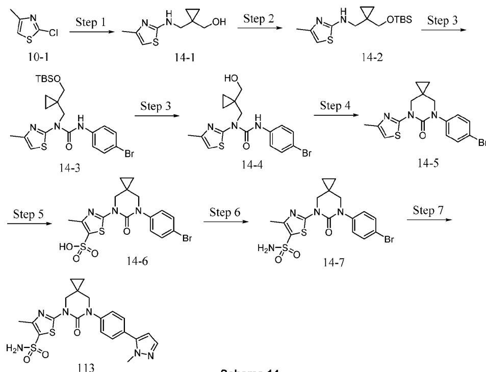
Scheme 14
