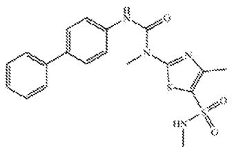
Example 123 WO200053591
