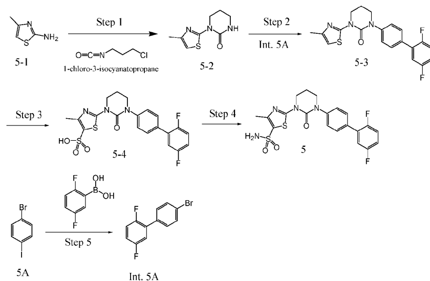
Scheme 22
