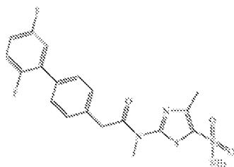
Example 87 WO2001047904
