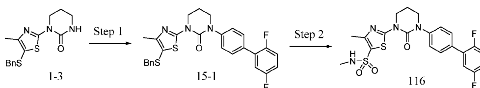
Scheme 15
