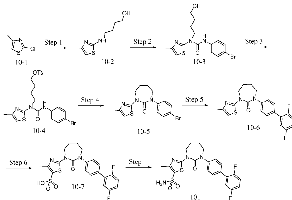
Scheme 10
