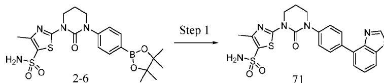
Scheme 8
