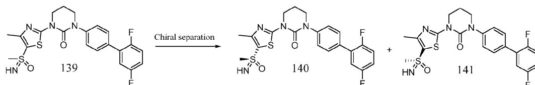
Scheme 17
