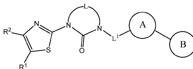
Formula II
