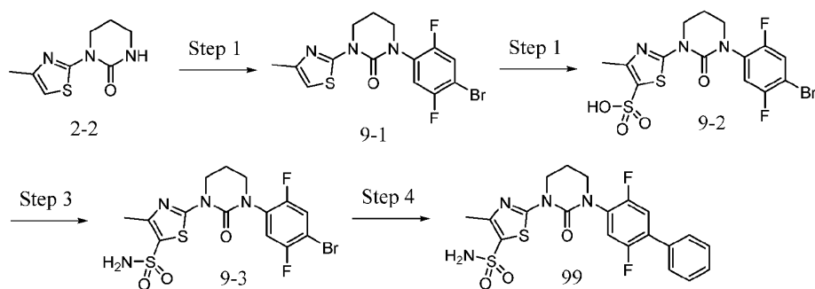
Scheme 9
