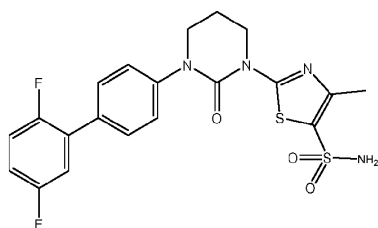
Example 5
