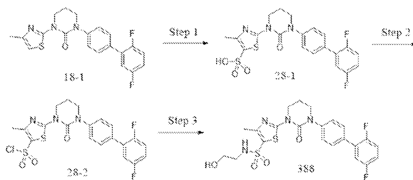
Scheme 28
