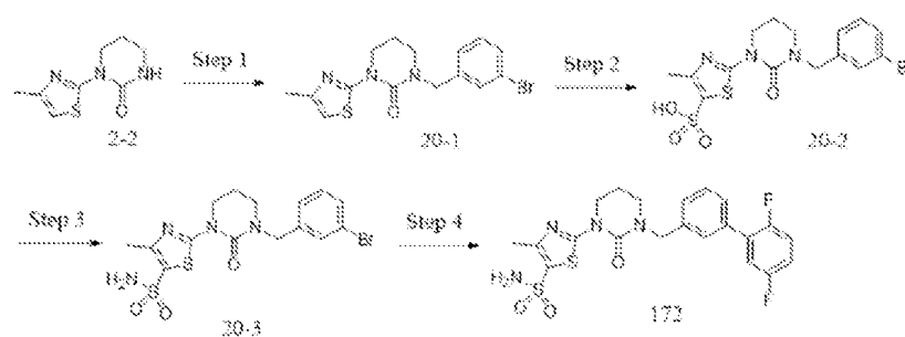
Scheme 20
