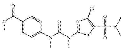
Example 38 WO200053591
