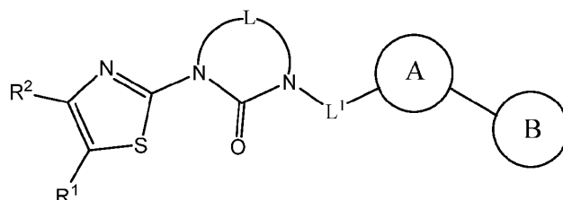
Formula II
