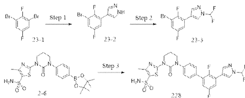
Scheme 23
