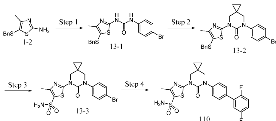
Scheme 13
