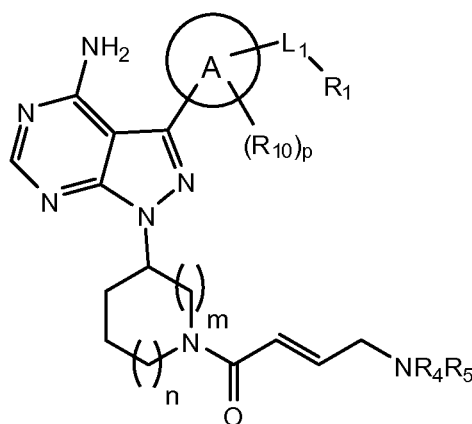
Formula (II);
