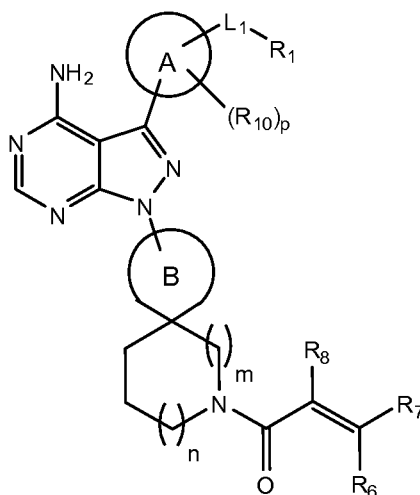
Formula (III);
