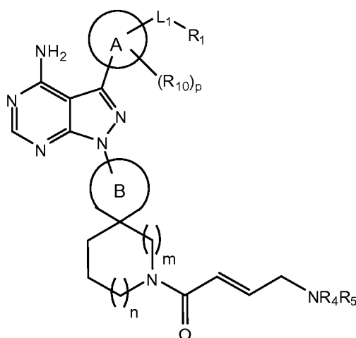
Formula (IIIa);
