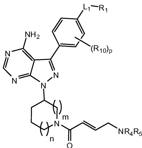
Formula (I);
