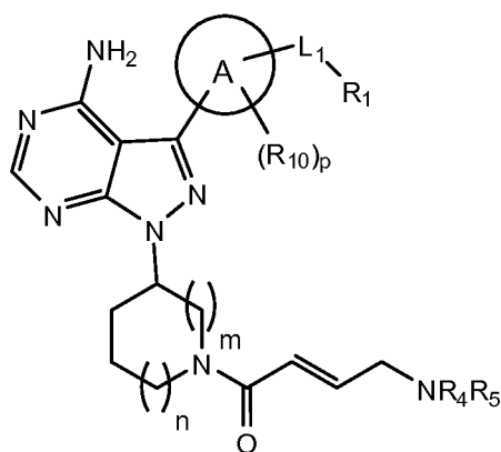
Formula (II);
