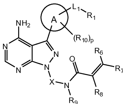
Formula (IV);
