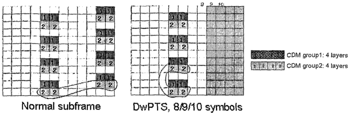
Figure 7 Extended CP rank 5-8 pattern: Option-1 with OCC=4
