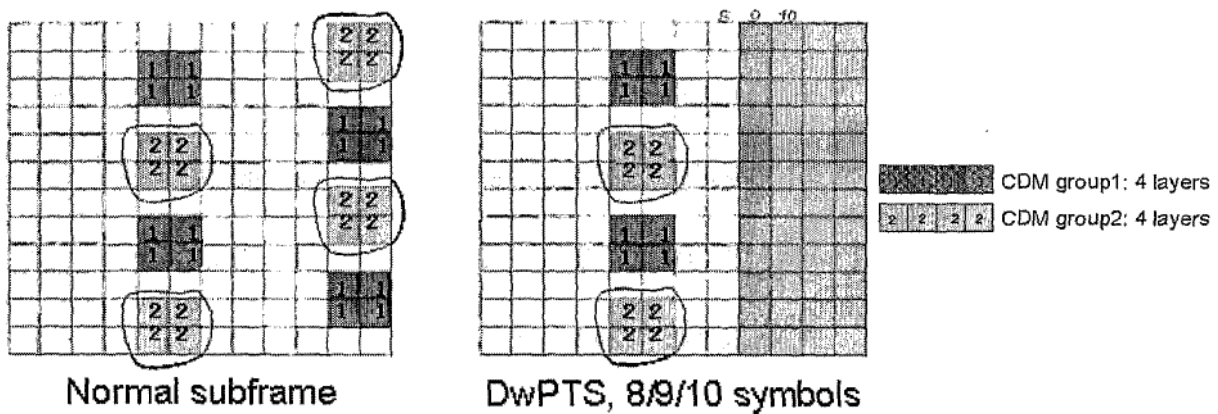
Figure 8 Extended CP rank 5-8 pattern: Option-2 with OCC=4
