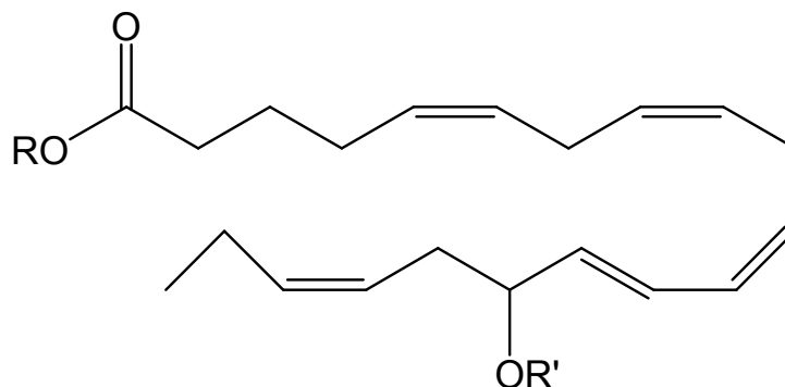
Formula (I)
