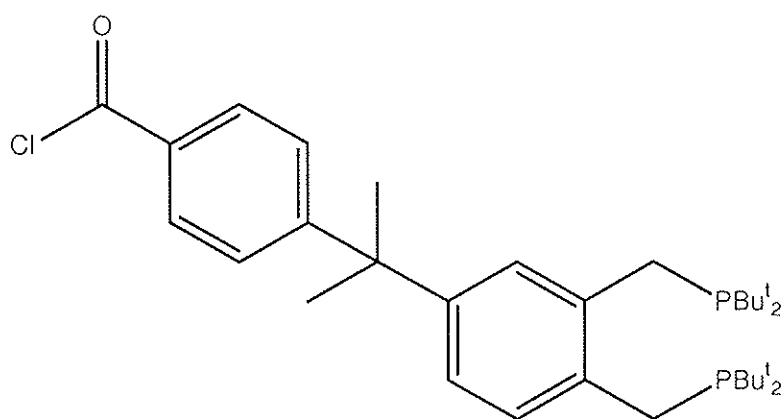
4-(1-{3,4-Bis-[(di-tert-butyl-phosphanyl)-methyl]-phenyl}-1-methyl-ethyl)-benzoyl chloride
