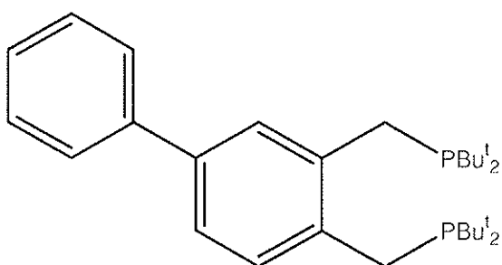
1,2-bis(di-tert-butyl(phosphinomethyl))-4-phenyl benzene
