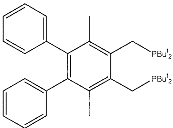
1,2-bis(di-tert-butyl(phosphinomethyl))-3,6-dimethyl-4,5-diphenyl benzene
