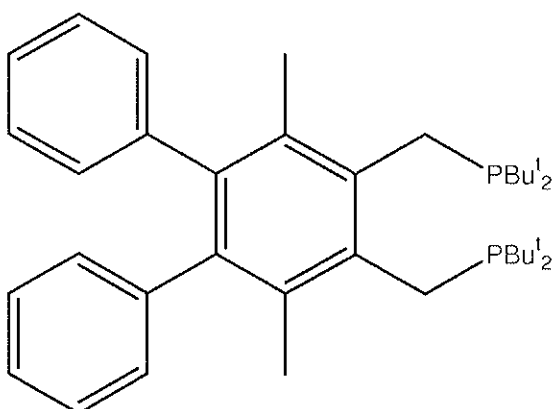
1,2-bis(di-tert-butyl(phosphinomethyl))-3,6-dimethyl-4,5-diphenyl benzene
