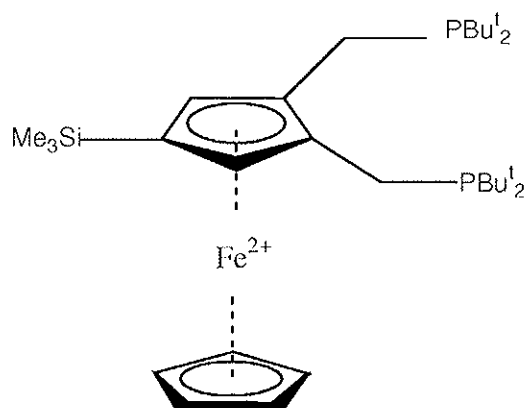
1,2-bis(di-tert-butylphosphinomethyl)-4-trimethylsilyl ferrocene
