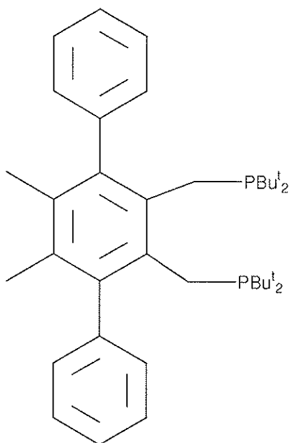
1,2-bis(di-tert-butylphosphinomethyl)-3,6-diphenyl-4,5-dimethylbenzene
