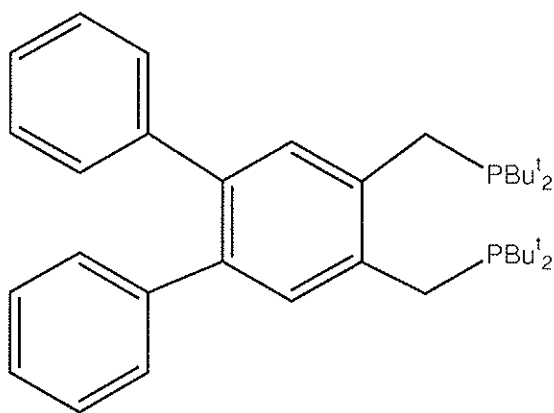
1,2 bis(di-tert-butyl(phosphinomethyl)-4,5-diphenyl 10 benzene
