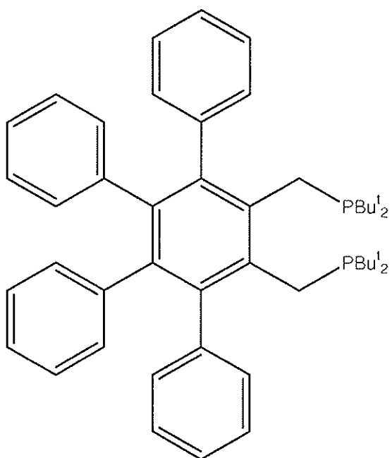
1,2-bis(di-tert-butyl(phosphinomethyl))-3,4,5,6-tetraphenyl benzene
