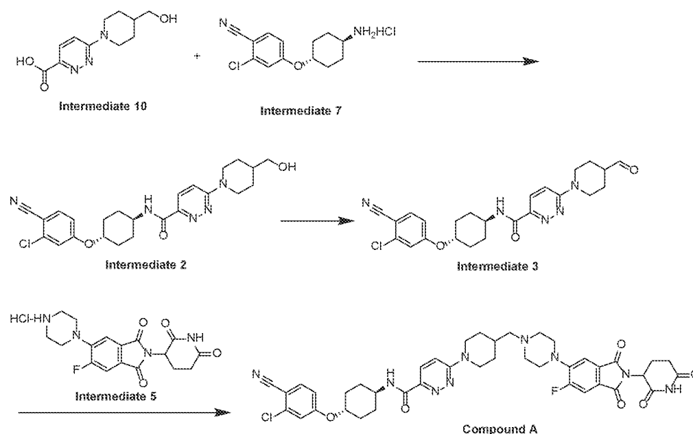
Scheme 6. Fourth Generation Manufacturing Process of Compound A
