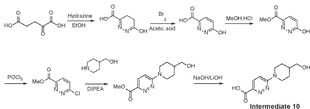
Scheme 7. Synthetic route to Intermediate 10
