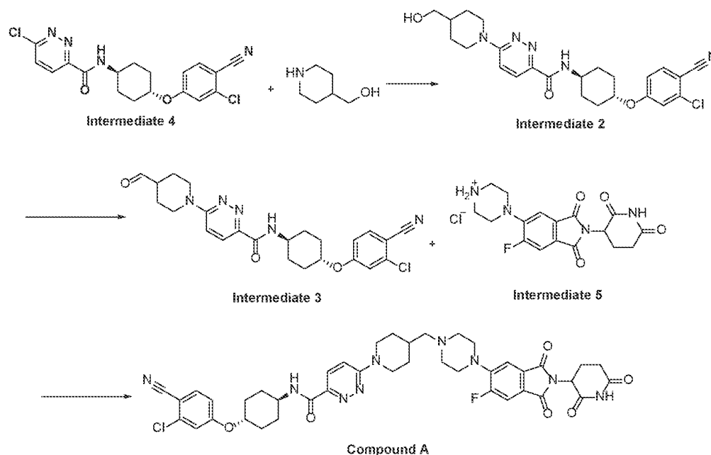
Scheme 4. Second Generation Manufacturing Process of Compound A
