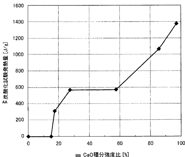
FIG. 1: AA Calorific value in carbonation test [J/g] BB Proportion of integrated intensity for CaO [%]
