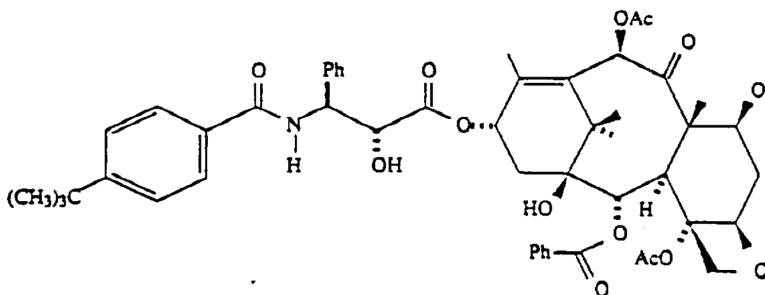
Preparation of N-debenzoyl-N-(4-t-butylbenzoyl) taxol
