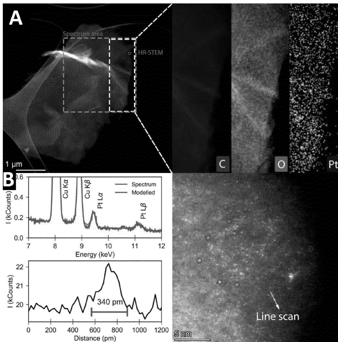
A) HAADF-STEM image of particles for mapping. Element mapping images of C, O, Pt with their overlapping images. B) STEM line scan, mapping size of single atom of Platinum
