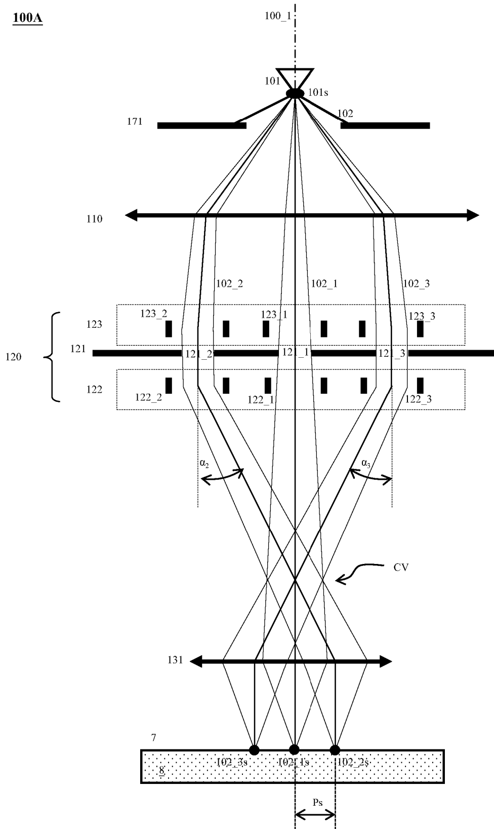
Figure 1A (Prior-Art)
