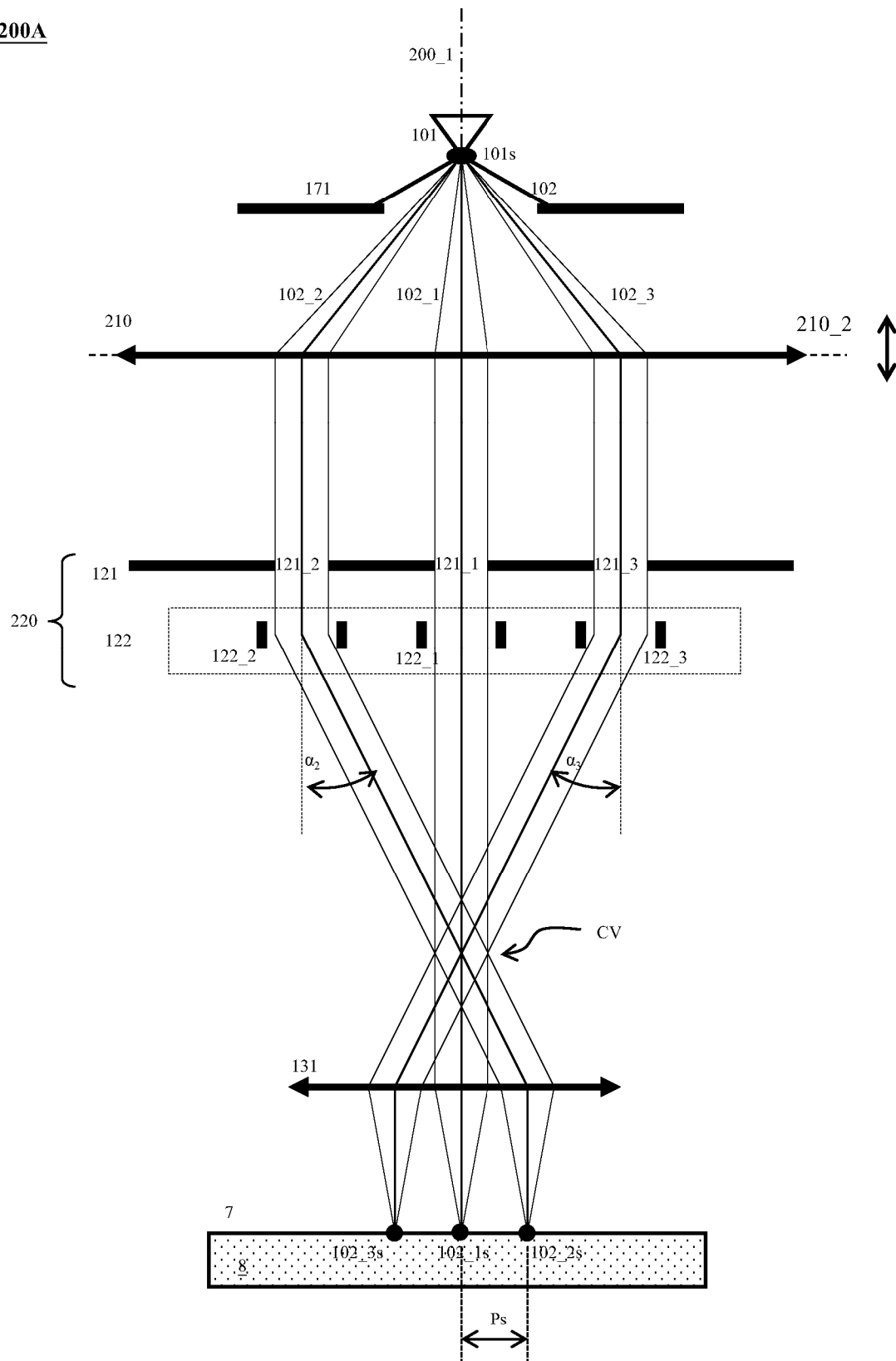
Figure 1B (Prior-Art)
