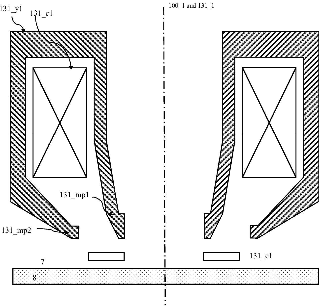
Figure 1C (Prior-Art)
