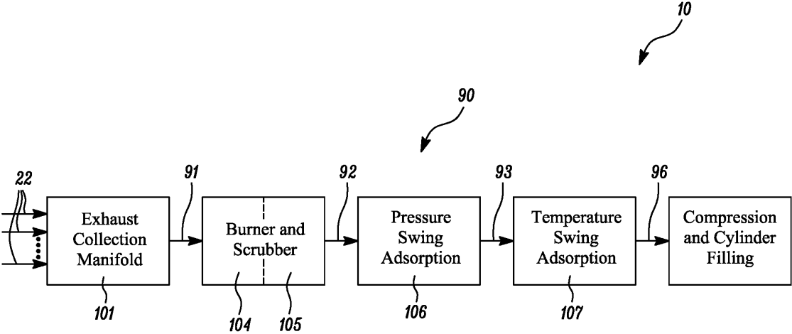
Xenon Recovery Integrated System: Major Unit Operations
