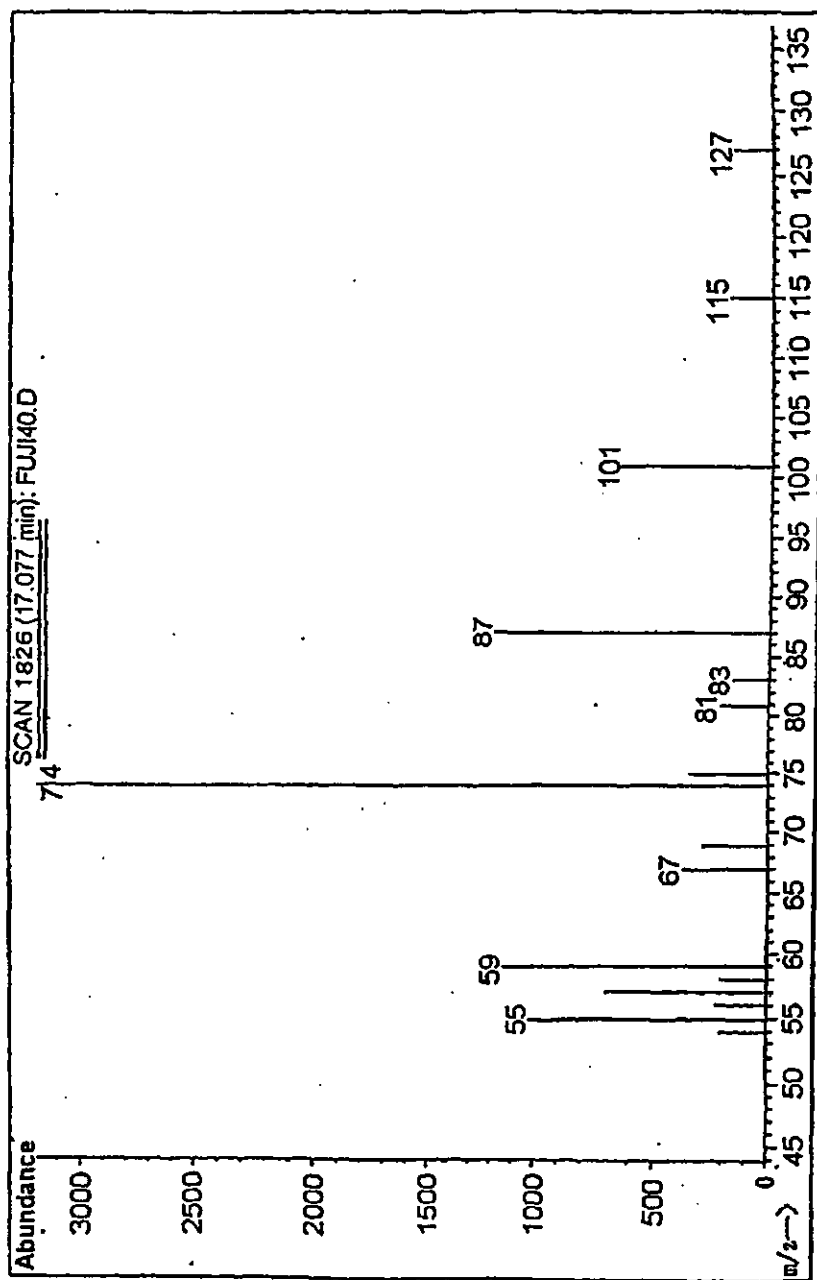
Figure 4 GC-MS DATA OF PURIFIED EUPHAUSIACEA SAMPLES
