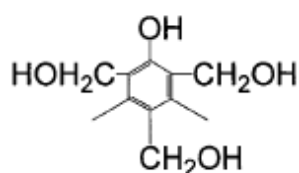
TriML-35XL
