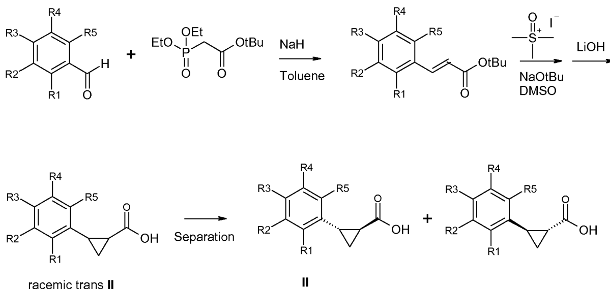
Scheme 3. Preparation of the (1 S , 2 S ) enantiomer of formula II.
