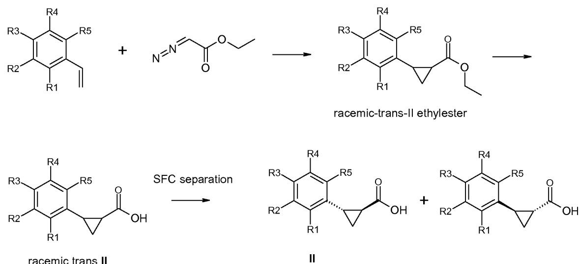
Scheme 2. Preparation of the (1S, 2S) enantiomer of formula II.
