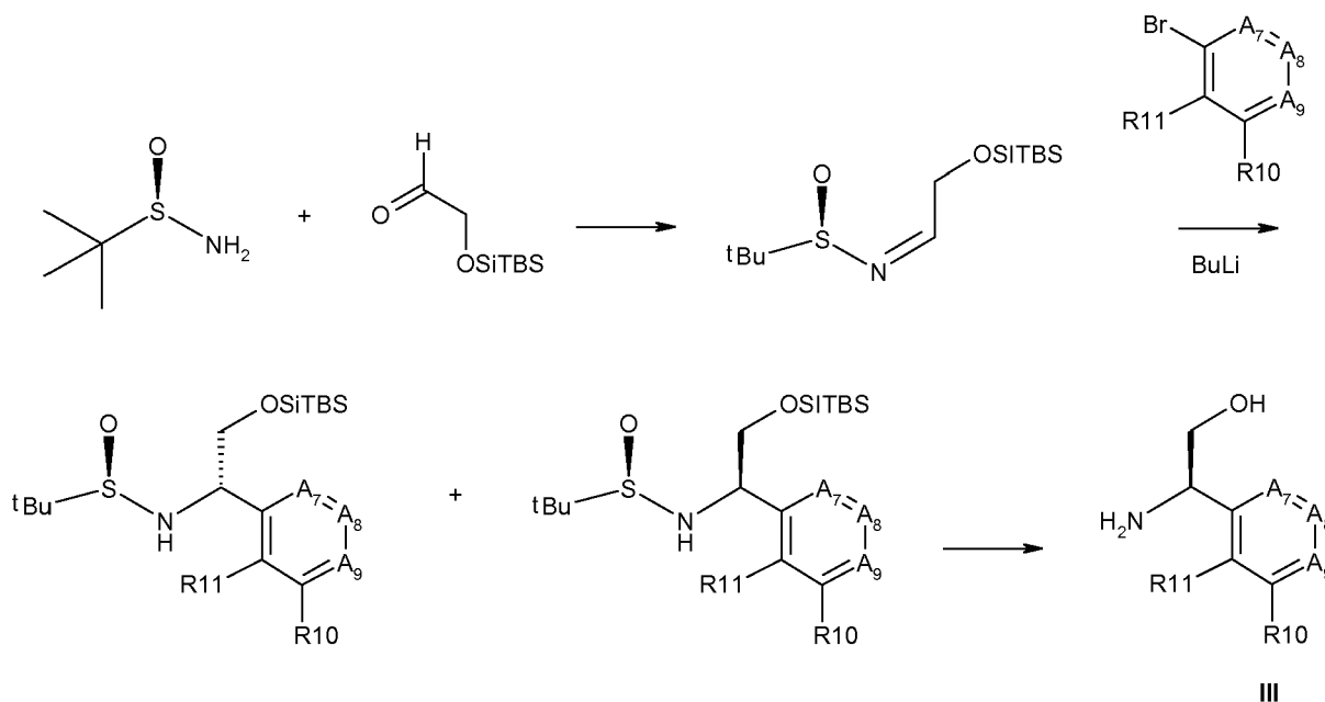
Scheme 4. Preparation of the chiral amines of formula III, with R_6 = CH_2OH . The method is described in: Barrow, J. C. et al. Tetrahedron Letters (2001) 2051.
