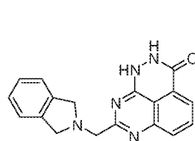
2X-121
