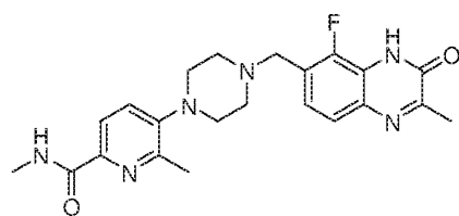
AZD9574
